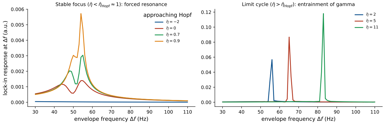
Figure 9: NMM2 PING gamma resonance (exact mean field). Lock-in response of the excitatory rate r_E at the envelope frequency \Delta f under an AM field (carrier 300 Hz). Left (stable focus, \bar{\eta} < \bar{\eta}_{\text{Hopf}} \approx 1 ): forced resonance at the gamma frequency ( f_0 \approx 55 Hz), growing as the Hopf is approached ( 1/\gamma gain), with the resonant frequency rising with \bar{\eta} . Right (limit cycle, \bar{\eta} > \bar{\eta}_{\text{Hopf}} ): entrainment of the autonomous gamma. The input carries no power at \Delta f ; the response is synthesized by the exact quadratic v^2 nonlinearity.
