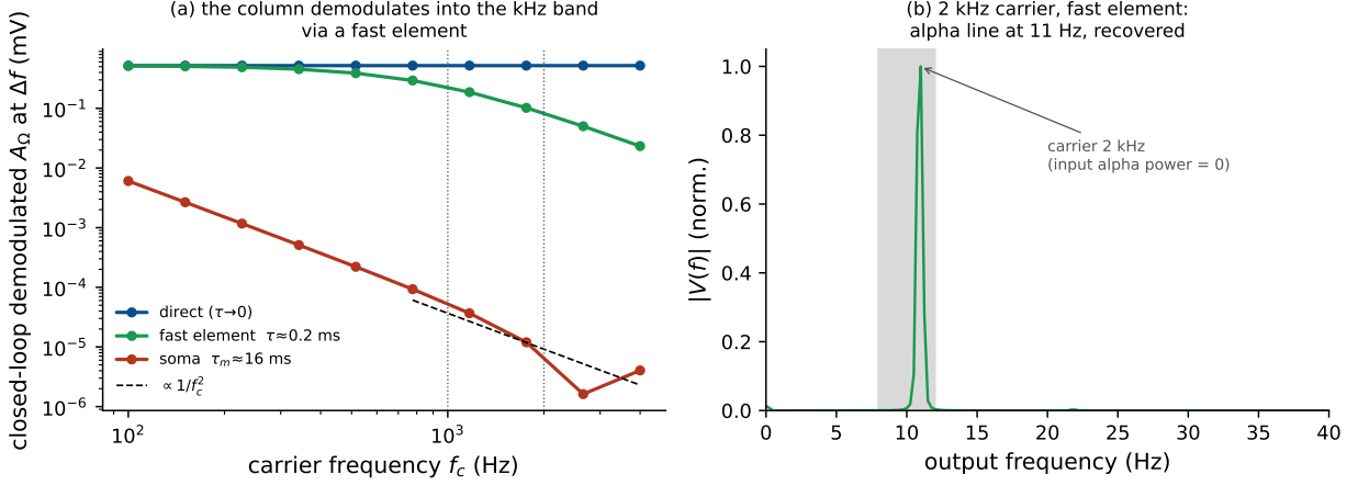
Figure 6: Demodulation at a genuine kHz carrier (Jansen–Rit, closed loop). The applied field passes through an explicit membrane filter before the sigmoid. (a) Closed-loop demodulated A_\Omega at \Delta f = f_0 vs. carrier f_c for three coupling routes: direct ( \tau \rightarrow 0 , carrier-independent), fast element (axon/AIS/node, \tau \approx 0.2 ms; survives into the kHz band), and soma ( \tau_m \approx 16 ms; collapses as 1/f_c^2 ). (b) Output spectrum for a 2 kHz carrier delivered through the fast element: a clean alpha line at f_0 , synthesized by the column although the input carries no alpha power.
