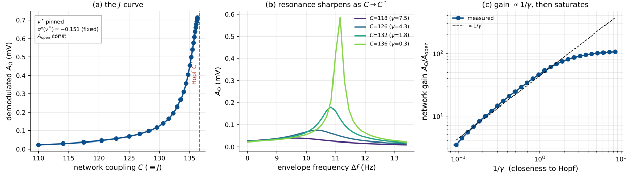
Figure 10: Coupling controls the amplification at fixed detection (Jansen–Rit). The operating point v^* is pinned by co-solving p(C) , so \sigma''(v^*) and A_{\text{open}} are constant. (a) The demodulated A_\Omega grows as the coupling C (=J) approaches the Hopf C^* from the stable-focus side ( \gamma > 0 ). (b) The envelope resonance sharpens and grows as C \rightarrow C^* . (c) The network gain A_\Omega/A_{\text{open}} follows 1/\gamma (dashed) and saturates near the bifurcation.
