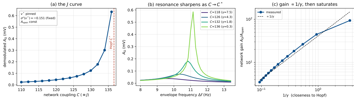
Figure 16: Coupling controls the amplification at fixed detection (Jansen–Rit). The operating point v^* is pinned by co-solving p(C) , so \sigma''(v^*) and A_{\text{open}} are constant. (a) The demodulated A_\Omega diverges as the coupling C (= J) approaches the Hopf C^* . (b) The envelope resonance sharpens and grows as C \rightarrow C^* . (c) The network gain A_\Omega/A_{\text{open}} follows 1/\gamma (dashed) and saturates near the bifurcation.
