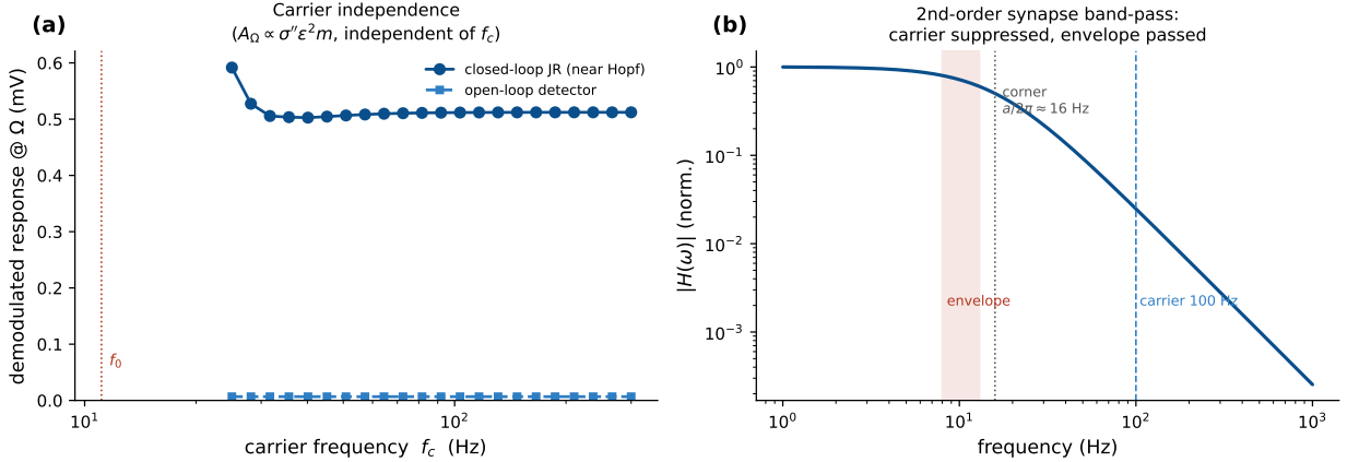
Figure 5: The demodulated response is carrier-independent at fixed polarization (Jansen–Rit). Left: the demodulated response is flat across carrier frequency f_c = 25 – 300 Hz, both for the open-loop detector (exactly, by Eq. (10)) and for the closed-loop JR near the Hopf (which adds \sim 60\times resonant gain); deviations appear only as f_c approaches the natural band. Right: the second-order-synapse band-pass |H(\omega)| passes the envelope ( \sim 0.7 ) and suppresses the 100 Hz carrier ( \sim 2.5\% ).
