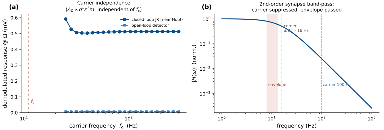
Figure 5: The demodulated response is carrier-independent at fixed polarization (Jansen–Rit). Left: the demodulated response is flat across carrier frequency f_c = 25 –300 Hz, both for the open-loop detector (exactly, by Eq. (10)) and for the closed-loop JR near the Hopf (which adds \sim 60\times resonant gain); deviations appear only as f_c approaches the natural band. Right: the second-order-synapse band-pass |H(\omega)| passes the envelope ( \sim 0.7 ) and suppresses the 100 Hz carrier ( \sim 2.5\% ).
