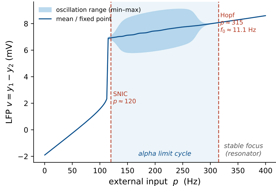
JR bifurcation diagram
