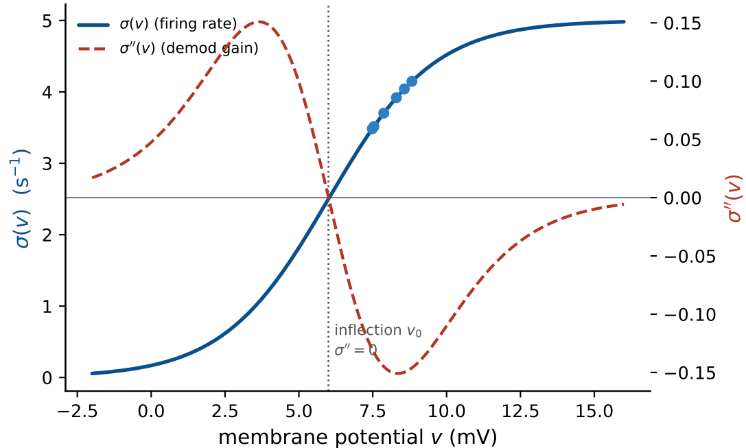
Sigmoid \sigma(v) and its curvature \sigma''
