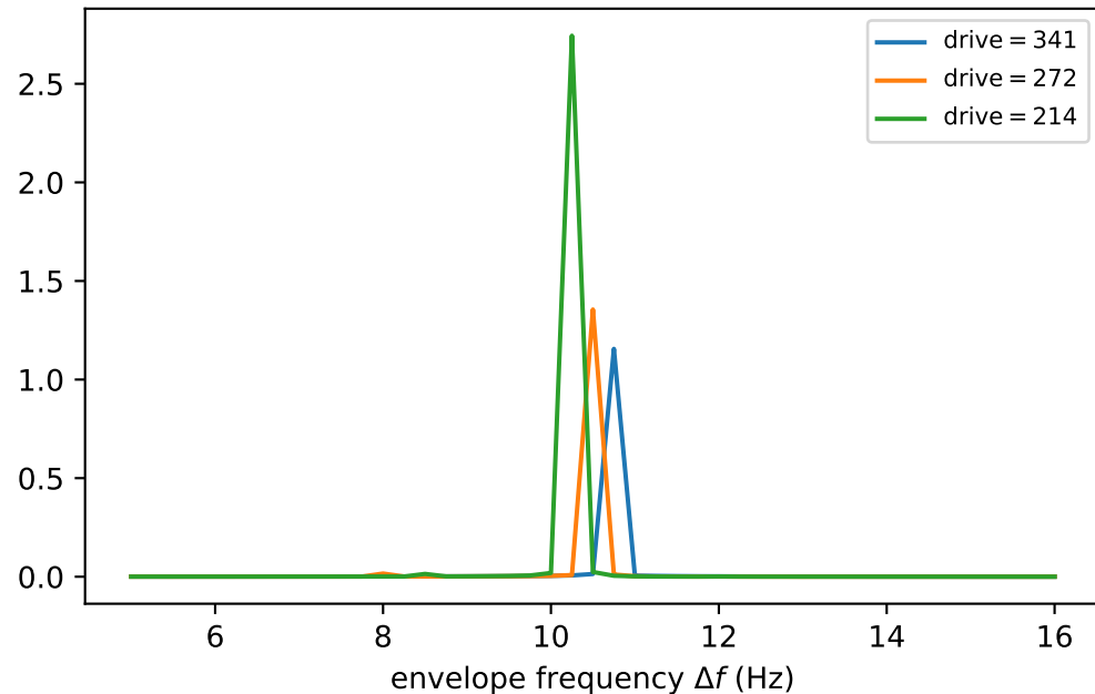
Limit cycle (low drive < Hopf): entrainment of alpha
