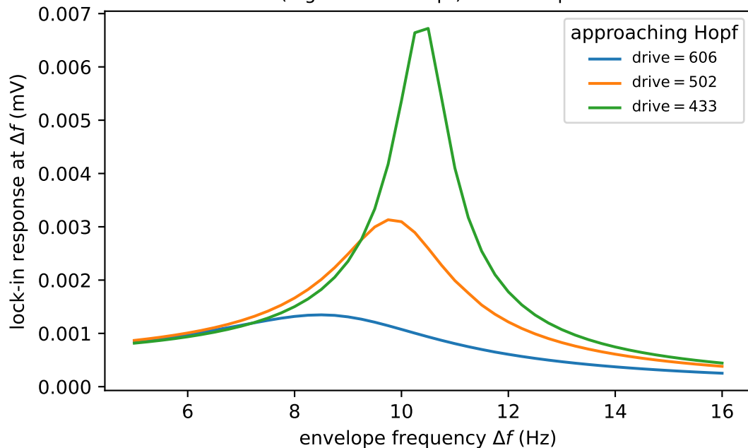
Stable focus (high drive > Hopf): forced alpha resonance
