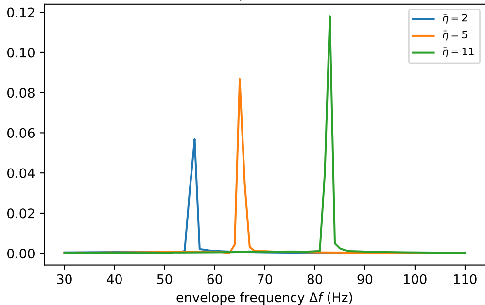
Limit cycle ( \bar{\eta} > \bar{\eta}_{\text{Hopf}} ): entrainment of gamma
