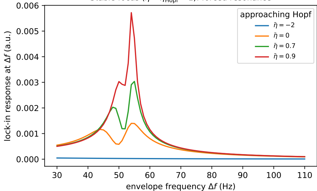
Stable focus ( \bar{\eta} < \bar{\eta}_{\text{Hopf}} \approx 1 ): forced resonance
