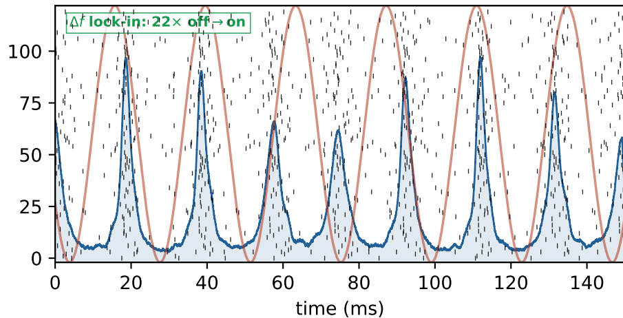
(d) Entrained, TI ON ( \Delta f=42 Hz): gamma bursts gate to the TI beat
