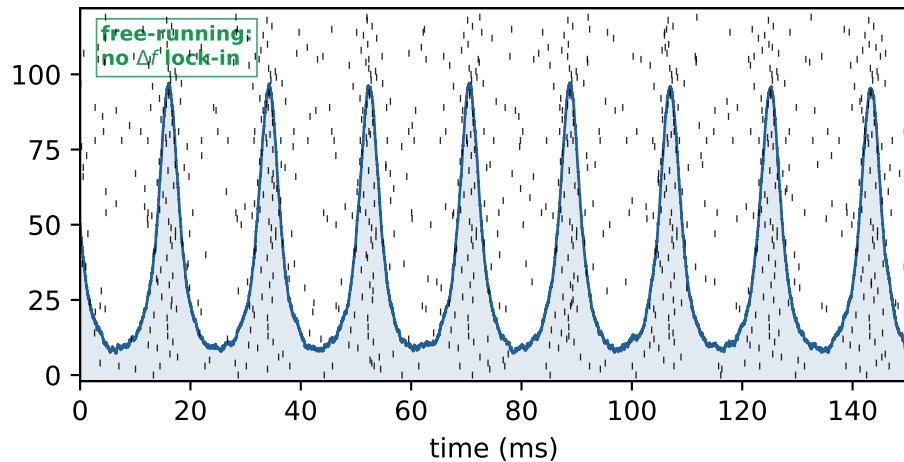
(c) Entrained (above Hopf), TI OFF: free gamma
