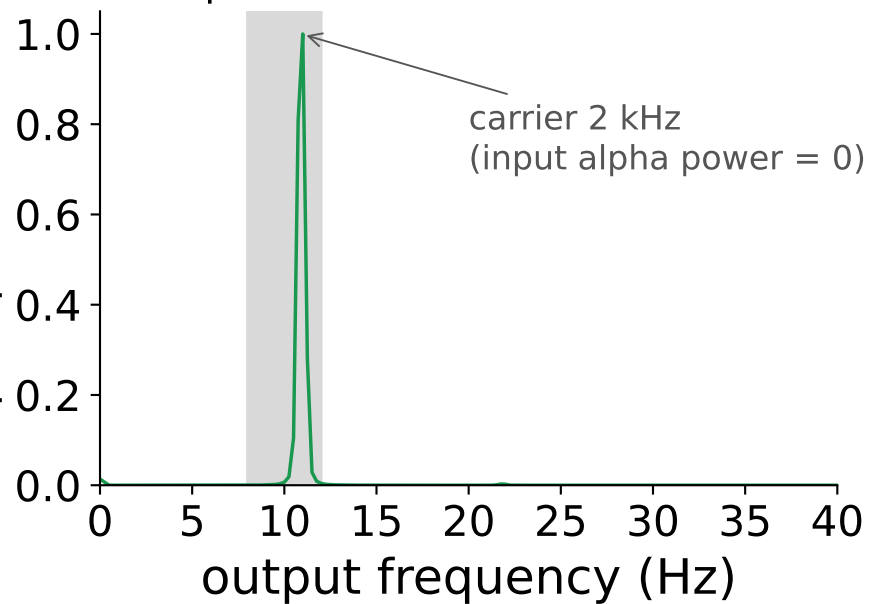
(b) 2 kHz carrier, fast element: alpha line at 11 Hz, recovered
