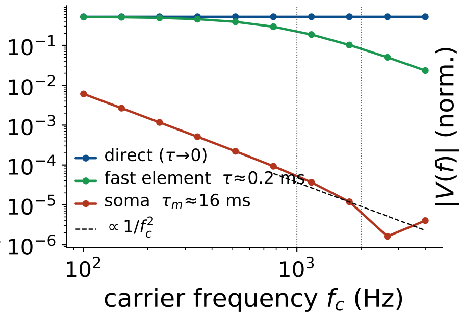
(a) the column demodulates into the kHz band via a fast element
