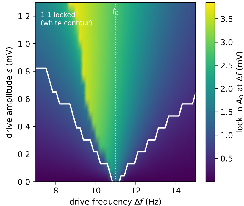
(a) 1:1 Arnold tongue (lock-in)
