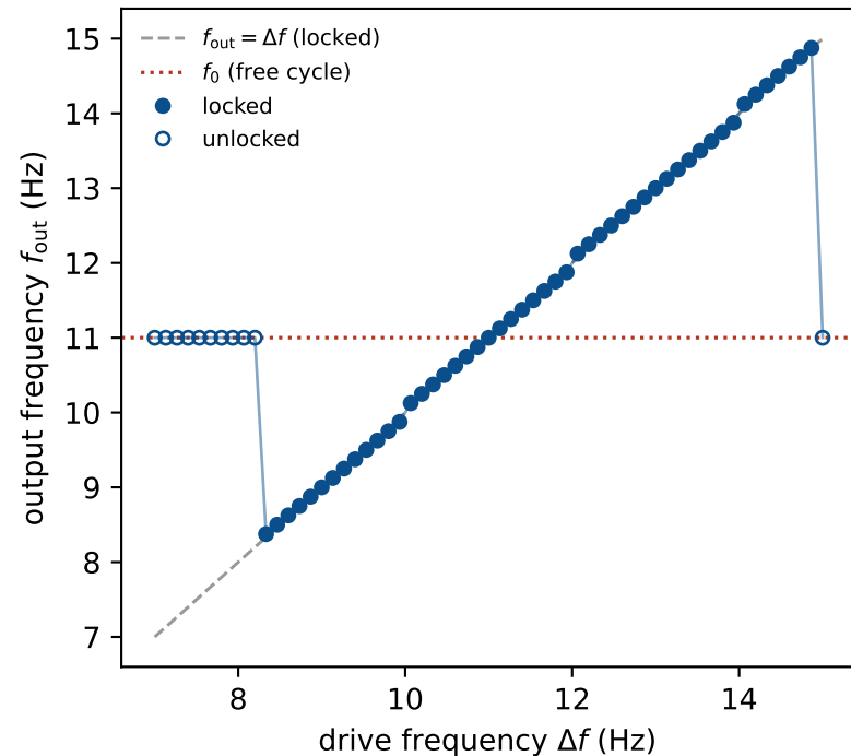
(b) frequency locking ( \varepsilon = 0.6 mV)
