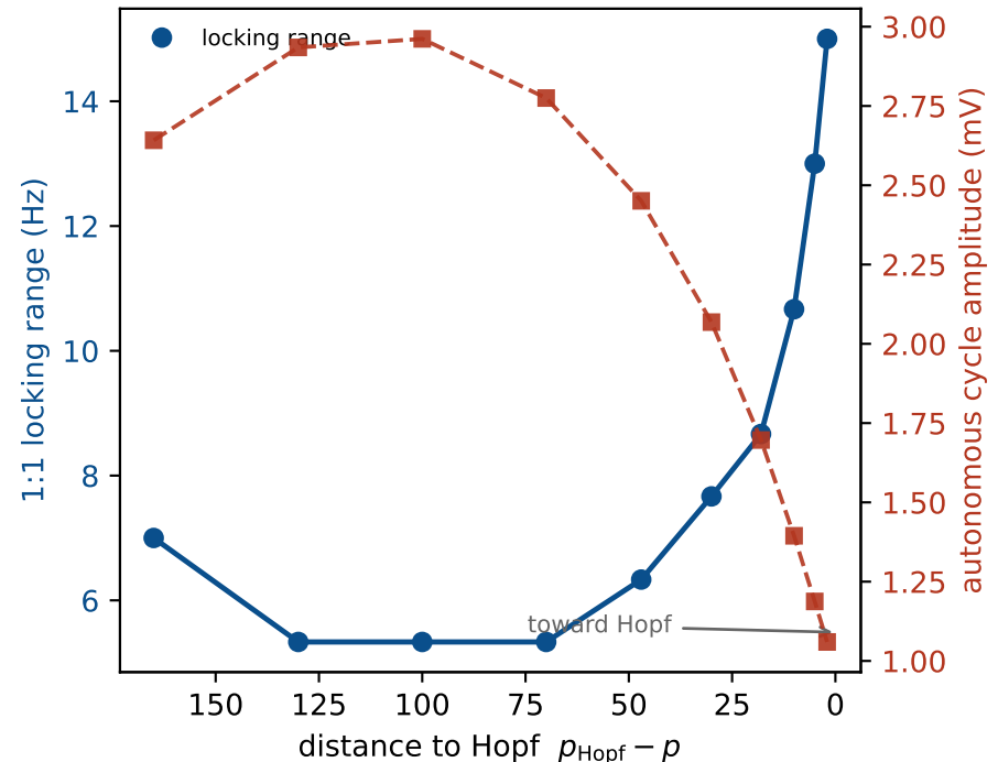
(c) entrainment grows toward criticality
