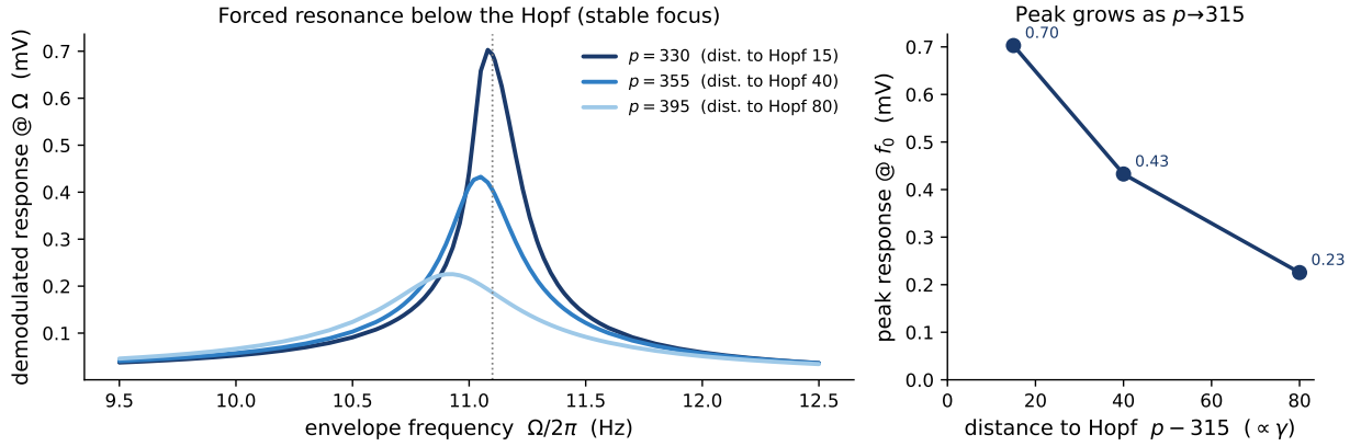
Figure 4: The recovered envelope drives a resonance that sharpens toward the Hopf (Jansen–Rit). Fixed-point regime ( p > 315 , stable focus): lock-in response at \Omega vs. envelope frequency ( \varepsilon = 0.3 mV). Left: the demodulated drive forces a Lorentzian resonance at f_0 \approx 11.1 Hz whose peak redshifts slightly as the damping grows ( \omega_{\text{peak}} = \sqrt{\omega_0^2 - 2\gamma^2} ; 11.08 \rightarrow 10.93 Hz across the three curves); the response carries no power at \Omega in the absence of drive, so this is genuine forced gain. Right: the peak height grows monotonically as the Hopf is approached ( p \rightarrow 315 , distance to Hopf \rightarrow 0 ), i.e. gain \propto 1/\gamma . The complementary above-Hopf regime, where the demodulated drive entrains the autonomous alpha within a 1:1 Arnold tongue, is characterized with the appropriate observable (output frequency f_{\text{out}} , not lock-in amplitude) in Fig. S5.
