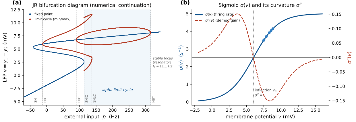
Figure 2: The Jansen–Rit operating regime: bifurcation and sigmoid curvature. Left: JR bifurcation diagram from numerical continuation—the LFP v = y_1 - y_2 along the fixed-point branch (blue) and the min/max of the limit-cycle branches (red) vs. external input p , with solid stable and faded unstable. The alpha limit cycle (shaded) is bounded by a saddle-node-on-invariant-circle (SNIC, p \approx 114 ) and the supercritical Hopf ( p \approx 315 , f_0 \approx 11.1 Hz); beyond the Hopf the fixed point is a stable focus—the near-critical resonator regime used throughout. The column is a weakly-damped focus near both bifurcations, so it resonates on either approach—more slowly near the SNIC. Further codim-1 points are marked (saddle-node SN, Hopf HB^\pm , saddle-node of limit cycles SNLC). Right: the sigmoid \sigma(v) and its curvature \sigma''(v) , which sets the demodulation gain and vanishes at the inflection v_0 . Dots mark the operating points reached by the closed-loop model for the p values used here.
