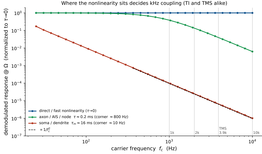
Figure S7: Somatic demodulation dies at kHz, but a fast element survives (Jansen–Rit, open-loop detector). Open-loop demodulated response (normalized to the \tau \rightarrow 0 value) vs. carrier frequency up to 10 kHz. With direct coupling ( \tau \rightarrow 0 ) the response is flat—carrier-independent. A slow somatic membrane ( \tau_m \approx 16 ms) rolls off as 1/f_c^2 (dashed guide), killing kHz demodulation; a fast element (axon/AIS/node, \tau \approx 0.2 ms) retains an appreciable response into the kHz band ( \sim 0.14 at 2 kHz, \sim 0.04 at the TMS peak 3.9 kHz). The same membrane filter attenuates TMS at the soma, which is why neither TMS nor TI should be thought of as driving the soma at kHz.
