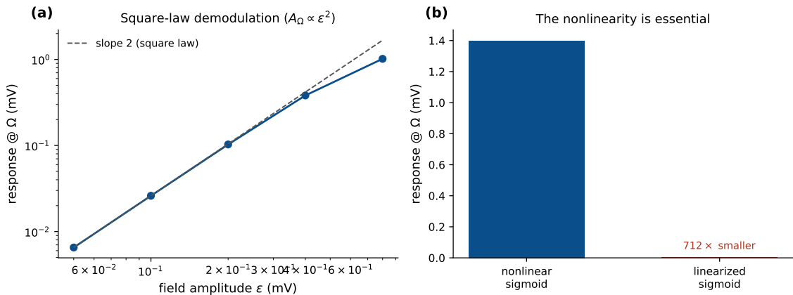
Figure S8: Verification (Jansen–Rit): square-law scaling and the linearization control. Left: response vs. field amplitude; small-drive log–log slope = 1.99 (theory 2). Right: linearizing the field-receiving sigmoid collapses the response 712\times ( 1.40 \rightarrow 0.0020 mV)—the nonlinearity is the demodulator.
