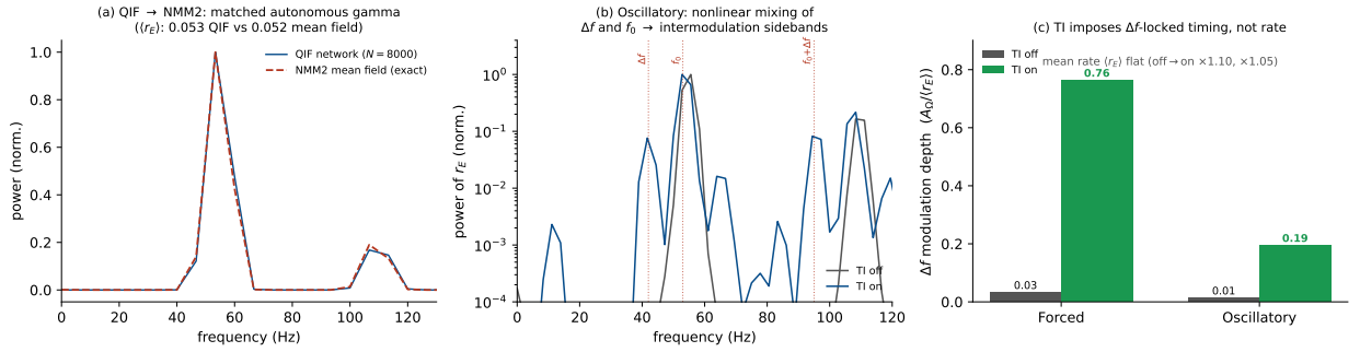
Figure S15: Timing, not rate, in the QIF network. (a) Power spectrum of r_E(t) in the field-free (autonomous) state: the spiking network ( N = 8000 ) matches the exact NMM2 mean field in the gamma rhythm (both \sim 53 Hz) and in mean rate \langle r_E \rangle . (b) Intermodulation in the oscillatory regime (TI off vs. on, log power): with TI on the nonlinearity mixes the imposed \Delta f = 42 Hz beat with the intrinsic f_0 \approx 53 Hz gamma, lighting up the direct \Delta f line and the sum sideband f_0 + \Delta f \approx 95 Hz, both absent when TI is off (the difference tone f_0 - \Delta f \approx 11 Hz sits near the floor, its amplitude set by the network transfer function rather than the mixer)—the spiking-network view of the same sigmoid frequency-mixing that drives demodulation throughout, and the sideband signature of gating rather than entrainment. (c) The \Delta f modulation depth A_\Omega/\langle r_E \rangle —the amplitude of the \Delta f -locked rate oscillation as a fraction of the mean rate—off vs. on: near zero with TI off (0.01–0.03), large with TI on (0.19 oscillatory, 0.76 forced), while the mean rate stays flat ( \times 1.05 – 1.10 ). We report the modulation depth rather than the off \rightarrow on lock-in ratio because the latter divides by the near-zero field-free baseline and is realization-noisy; the depth uses two well-estimated quantities and is stable.
