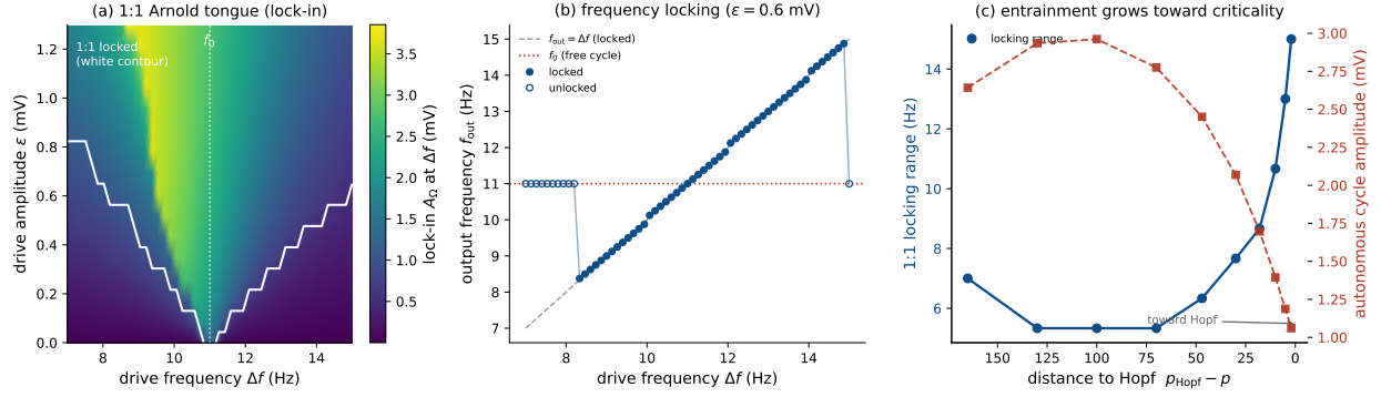
Figure S5: Above the Hopf: entrainment, not 1/\gamma amplification (Jansen–Rit). The column is set in its autonomous alpha limit cycle (input p = 250 , below the input Hopf; f_0 \approx 11 Hz) and driven by a direct in-band sinusoid at \Delta f . (a) The 1:1 Arnold tongue—the region of (\Delta f, \varepsilon) where the dominant output frequency locks to \Delta f —is a wedge anchored at f_0 that widens with drive amplitude. (b) Frequency locking at fixed drive: inside the tongue the output follows \Delta f (diagonal); outside, it falls back to the autonomous f_0 . (c) Sweeping the operating point toward the Hopf at fixed drive, the locking range (tongue width) grows as the autonomous cycle amplitude \rightarrow 0 : entrainment is easiest near criticality—the supercritical counterpart of the 1/\gamma forced gain. Here amplification is read as entrainment (tongue width, locking range), not as the diverging 1/\gamma gain of the stable-focus side (Fig. 9)—so the column is most responsive near criticality on both sides of the Hopf: to forcing below, to entrainment above.
