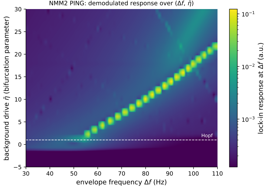
Figure S11: NMM2 PING resonance map (exact mean field). Demodulated response over the (envelope frequency \Delta f , background drive \bar{\eta} ) plane (log color scale: entrainment far exceeds the stable-focus forced response). The ridge follows the gamma natural frequency f_0(\bar{\eta}) and intensifies through the supercritical Hopf (dashed line); its diagonal slope— f_0 rising with \bar{\eta} —reflects the state-dependent transfer of NMM2, absent in the static-sigmoid JR and LaNMM.
