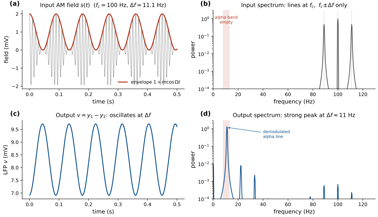
Figure 3: An alpha rhythm is synthesized from a carrier-only input (Jansen–Rit below Hopf). Top left: the AM field s(t) and its envelope. Top right: the input spectrum has lines only at f_c and f_c \pm \Delta f (89, 100, 111 Hz); the alpha band (shaded) is empty. Bottom left: the output v = y_1 - y_2 oscillates at the envelope frequency. Bottom right: the output spectrum has a strong peak at \Omega \approx 11 Hz, synthesized by the sigmoid and absent from the input.
