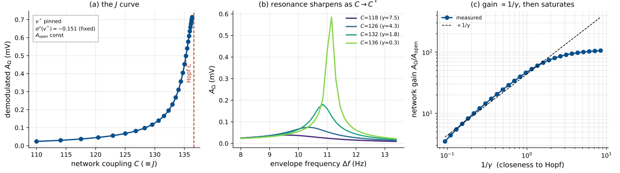
Figure 9: Coupling controls the amplification at fixed detection (Jansen–Rit). The operating point v^* is pinned by co-solving p(C) , so \sigma''(v^*) and A_{\text{open}} are constant. (a) The demodulated A_\Omega grows as the coupling C (= J) approaches the Hopf C^* from the stable-focus side ( \gamma > 0 ). (b) The envelope resonance sharpens and grows as C \rightarrow C^* . (c) The network gain A_\Omega/A_{\text{open}} follows 1/\gamma (dashed) and saturates near the bifurcation.
