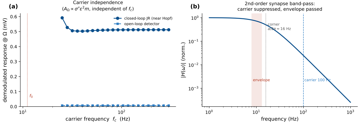
Figure 5: The demodulated response is carrier-independent at fixed polarization (Jansen–Rit). Left: the demodulated response is flat across carrier frequency f_c = 25\text{--}300 Hz, both for the open-loop detector (exactly, by Eq. (10)) and for the closed-loop JR near the Hopf (which adds \sim 60\times resonant gain); deviations appear only as f_c approaches the natural band. Right: the second-order-synapse band-pass |H(\omega)| passes the envelope ( \sim 0.7 ) and suppresses the 100 Hz carrier ( \sim 2.5\% ).
