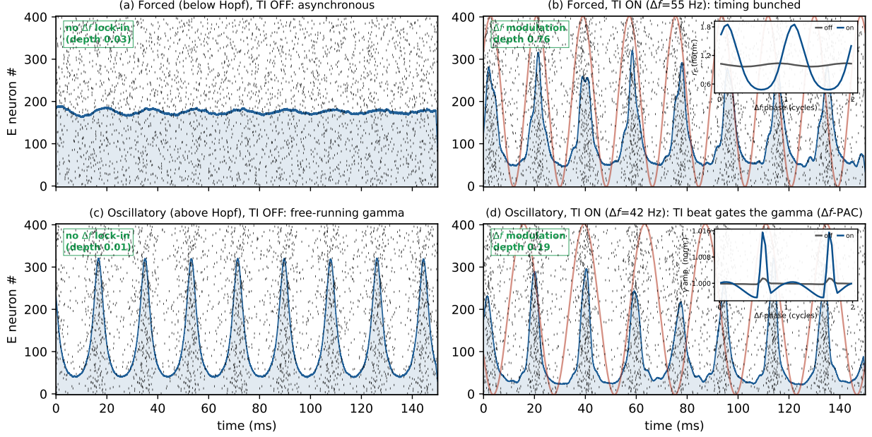
Figure 10: QIF spiking network (microscale of the NMM2 PING gamma generator): TI realigns spike timing, not mean rate. N = 8000 excitatory and inhibitory quadratic integrate-and-fire neurons whose exact mean field is the NMM2 PING circuit (Eq. (16)). This circuit’s intrinsic rhythm is gamma ( \sim 53 Hz), so, as in the alpha figures but one band up, the TI beat \Delta f is set in the gamma range (here much larger than the \Delta f \sim 11 Hz of the Jansen–Rit alpha column; carrier f_c = 300 Hz). Black ticks are E spikes (400 of 8000, a representative sample), blue the population rate r_E(t) , red the TI envelope; the boxed value is the \Delta f modulation depth A_\Omega/\langle r_E \rangle of the rate (near zero off, large on). The bifurcation parameter is the common background drive \bar{\eta} (gamma Hopf at \bar{\eta}_{\text{Hopf}} \approx 1.1 ). (a) Forced ( \bar{\eta} = 0.85 , just below the Hopf—a damped gamma resonator), TI off: asynchronous firing, flat rate. (b) Forced, TI on, driven near the gamma resonance ( \Delta f = 55 Hz): spikes bunch into the envelope (modulation depth 0.76). (c) Oscillatory ( \bar{\eta} = 1.5 , above the Hopf—an autonomous \sim 53 Hz gamma cycle), TI off: free-running gamma, no \Delta f lock-in. (d) Oscillatory, TI on, with the beat set below the autonomous gamma (beat \Delta f = 42 Hz, a detuning of \approx 11 Hz from f_0 \approx 53 Hz): the TI beat gates the gamma—the population rate gains a \Delta f -locked component (modulation depth 0.19) while the intrinsic \sim 53 Hz gamma persists. This is forced cross-frequency gating (PAC), not frequency entrainment: the \sim 11 Hz detuning places the beat outside the 1:1 Arnold tongue (contrast the genuine frequency locking of Fig. S5), so the gamma is amplitude-modulated at \Delta f rather than pulled to it—demodulation surviving above the Hopf as envelope-to-rhythm coupling. The detuning is what certifies the \Delta f -locked component as a real driven effect rather than coincidence. Insets (each normalized to its own mean, so the y -axis reads the relative modulation; x -axis is the \Delta f beat phase in cycles; TI off gray, on blue): (b) the population rate folded on the beat phase (the forced response is at \Delta f ); (d) the gamma-band amplitude folded on the beat phase—taking the amplitude removes the gamma carrier, so the near-commensurate 53/42 Hz gamma cannot contaminate the fold (a raw-rate fold would). Both are flat with TI off and show a clear \Delta f -locked modulation with TI on, making the envelope-locked timing direct where the raster alone leaves it subtle.
