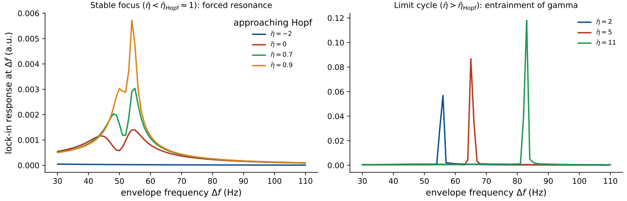
Figure 8: NMM2 PING gamma resonance (exact mean field). Lock-in response of the excitatory rate r_E at the envelope frequency \Delta f under an AM field (carrier 300 Hz). Left (stable focus, \bar{\eta} < \bar{\eta}_{\text{Hopf}} \approx 1 ): forced resonance at the gamma frequency ( f_0 \approx 55 Hz), growing as the Hopf is approached ( 1/\gamma gain), with the resonant frequency rising with \bar{\eta} . Right (limit cycle, \bar{\eta} > \bar{\eta}_{\text{Hopf}} ): entrainment of the autonomous gamma. The input carries no power at \Delta f ; the response is synthesized by the exact quadratic v^2 nonlinearity.
