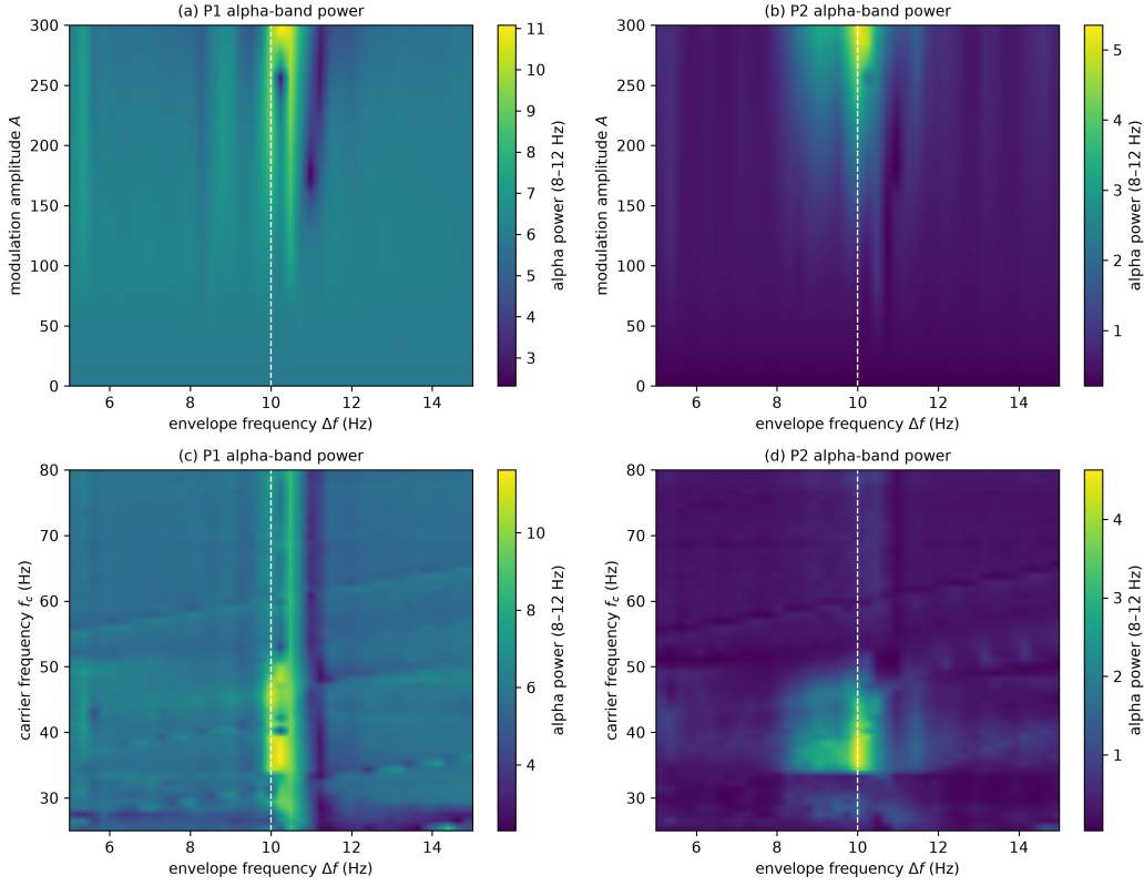
Figure 7: LaNMM Arnold tongues: AM input to the superficial P_2 (gamma) loop. (a,b) Alpha-band power of P_1 and P_2 vs. modulation amplitude A and beat frequency \Delta f (carrier 40 Hz): a tongue of elevated power around the P_1 alpha ( \sim 10 Hz, dashed line) that widens with A . (c,d) Alpha power vs. carrier frequency and \Delta f at A = 250 : P_1 demodulation requires both a carrier \approx 40 Hz ( P_2 gamma) and \Delta f \approx 10 Hz ( P_1 alpha)—a double resonance.
