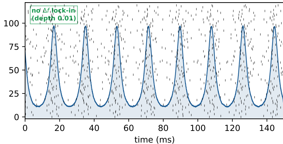
(c) Oscillatory (above Hopf), TI OFF: free-running gamma
