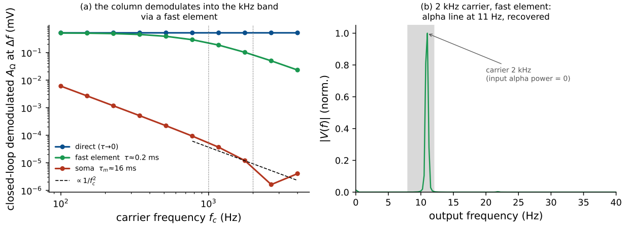
Figure 6: Demodulation at a genuine kHz carrier (Jansen–Rit, closed loop). The applied field passes through an explicit membrane filter before the sigmoid. (a) Closed-loop demodulated A_\Omega at \Delta f = f_0 vs. carrier f_c for three coupling routes: direct ( \tau \rightarrow 0 , carrier-independent), fast element (axon/AIS/node, \tau \approx 0.2 ms; survives into the kHz band), and soma ( \tau_m \approx 16 ms; collapses as 1/f_c^2 ). (b) Output spectrum for a 2 kHz carrier delivered through the fast element: a clean alpha line at f_0 , synthesized by the column although the input carries no alpha power.
