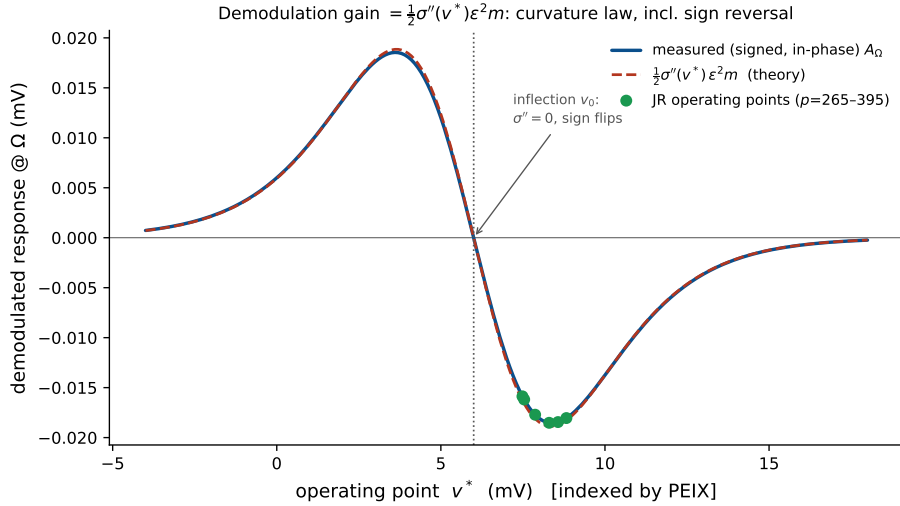
Figure 7: Operating-point law and the \sigma'' control (Jansen–Rit). The measured signed (in-phase) open-loop response tracks \frac{1}{2}\sigma''(v^*)\epsilon^2 m across the whole range, vanishes at the inflection v_0 , and reverses sign across it—a direct verification that demodulation is the sigmoid-curvature term of Eq. (10). The closed-loop JR operating points (dots) sit on the lobe where \sigma'' is large and negative—not by design, but because that is where the JR resting point lies as the alpha Hopf is approached (the saturating upper flank of the sigmoid). The mechanism is sign-agnostic: \sigma'' sets only the sign/phase of the demodulated response while |\sigma''| sets its gain, so the entire resonance picture is unchanged (up to an overall sign) in the \sigma'' > 0 lobe, which this open-loop sweep already spans. The sign flip itself is a falsifiable prediction (§4.10).
