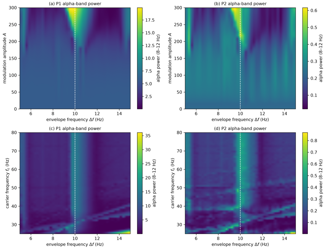
Figure S10: LaNMM envelope-resonance maps: AM input delivered directly to the deep P_1 (alpha) loop. (a,b) Alpha power of P_1 and P_2 vs. amplitude A and \Delta f . (c,d) Alpha power vs. carrier frequency and \Delta f : P_1 responds across a broad carrier band (a vertical ridge at \Delta f \approx 10 Hz)—carrier-independent, the direct-coupling limit of Eq. (10).
