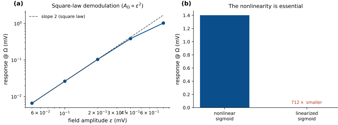
Figure S8: Verification (Jansen–Rit): square-law scaling and the linearization control. (a) Response vs. field amplitude; small-drive log–log slope = 1.99 (theory 2). (b) Linearizing the field-receiving sigmoid collapses the response 712 \times ( 1.40 \rightarrow 0.0020 mV)—the nonlinearity is the demodulator.
