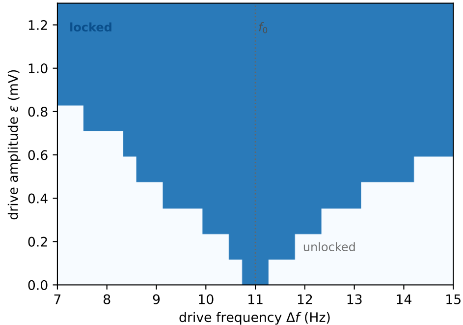
(a) 1:1 Arnold tongue (autonomous \alpha )
