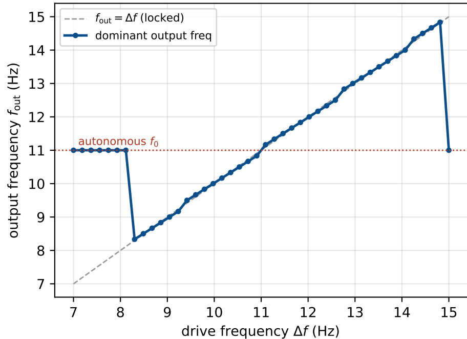
(b) frequency locking ( \varepsilon=0.6 )
