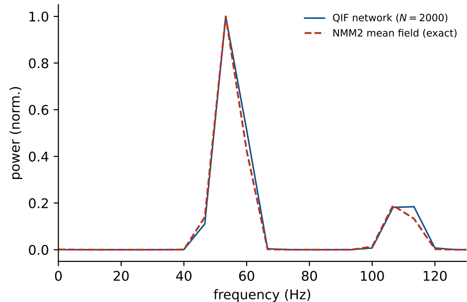
(a) QIF \rightarrow NMM2: matched autonomous gamma ( \langle r_E \rangle : 0.052 QIF vs 0.052 mean field)
