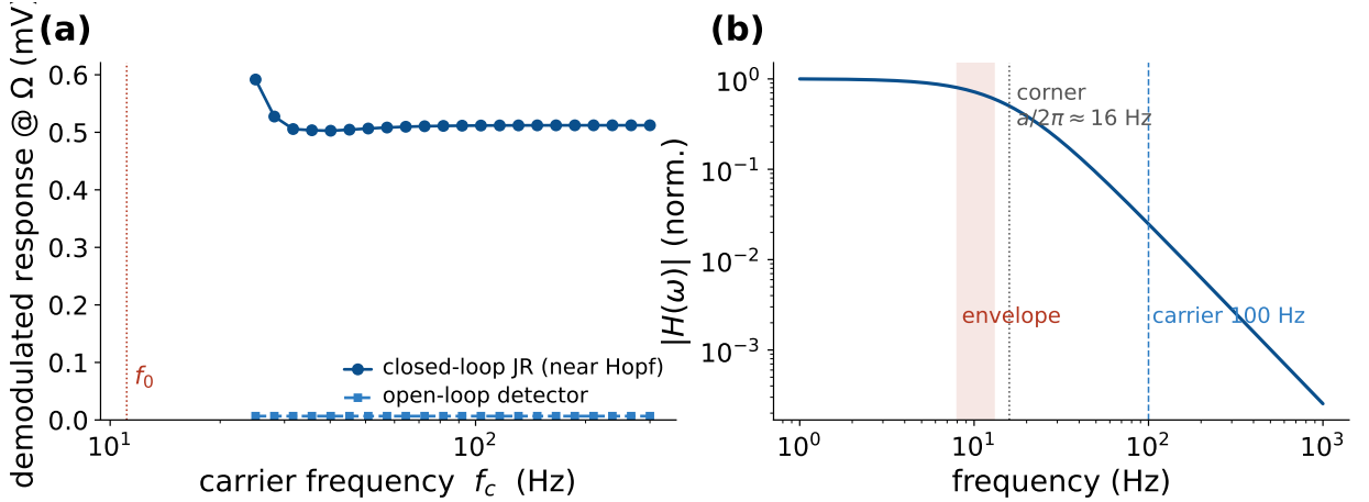
Figure 5: The demodulated response is carrier-independent at fixed polarization (Jansen–Rit). (a) The demodulated response is flat across carrier frequency f_c = 25 – 300 Hz, both for the open-loop detector (exactly, by Eq. (10)) and for the closed-loop JR near the Hopf (which adds \sim 60\times resonant gain); deviations appear only as f_c approaches the natural band. (b) The second-order-synapse band-pass |H(\omega)| passes the envelope ( \sim 0.7 ) and suppresses the 100 Hz carrier ( \sim 2.5\% ).
