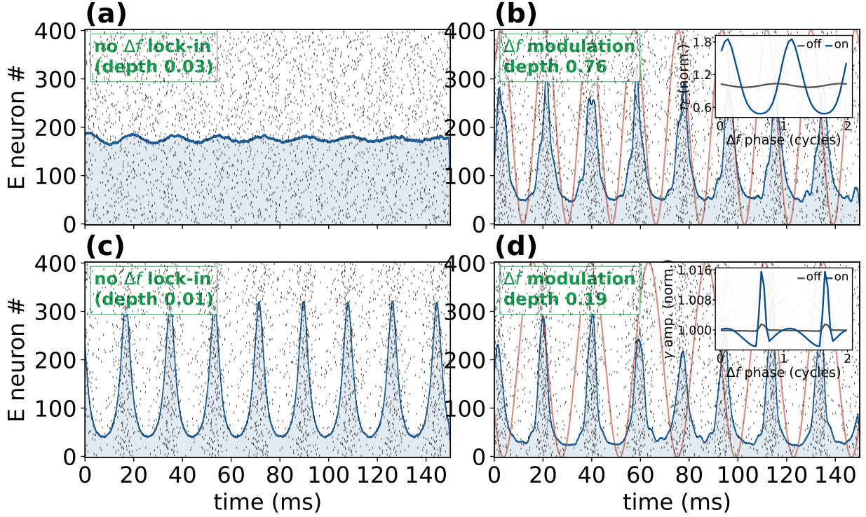
Figure 10: QIF spiking network (microscale of the NMM2 PING gamma generator): TI realigns spike timing, not mean rate. N = 8000 excitatory and inhibitory quadratic integrate-and-fire neurons whose exact mean field is the NMM2 PING circuit (Eq. (16)). This circuit’s intrinsic rhythm is gamma ( \sim 53 Hz), so, as in the alpha figures but one band up, the TI beat \Delta f is set in the gamma range (here much larger than the \Delta f \sim 11 Hz of the Jansen–Rit alpha column; carrier f_c = 300 Hz). Black ticks are E spikes (400 of 8000, a representative sample), blue the population rate r_E(t) , red the TI envelope; the boxed value is the \Delta f modulation depth A_\Omega/\langle r_E \rangle of the rate (near zero off, large on). The bifurcation parameter is the common background drive \bar{\eta} (gamma Hopf at \bar{\eta}_{\text{Hopf}} \approx 1.1 ). (a) Forced ( \bar{\eta} = 0.85 , just below the Hopf—a damped gamma resonator), TI off: asynchronous firing, flat rate. (b) Forced, TI on, driven near the gamma resonance ( \Delta f = 55 Hz): spikes bunch into the envelope (modulation depth 0.76). (c) Oscillatory ( \bar{\eta} = 1.5 , above the Hopf—an autonomous \sim 53 Hz gamma cycle), TI off: free-running gamma, no \Delta f lock-in. (d) Oscillatory, TI on, with the beat set below the autonomous gamma (beat \Delta f = 42 Hz, a detuning of \approx 11 Hz from f_0 \approx 53 Hz): the TI beat gates the gamma—the population rate gains a \Delta f -locked component (modulation depth 0.19) while the intrinsic \sim 53 Hz gamma persists. This is forced cross-frequency gating (PAC), not frequency entrainment: the \sim 11 Hz detuning places the beat outside the 1:1 Arnold tongue (contrast the genuine frequency locking of Fig. S5), so the gamma is amplitude-modulated at \Delta f rather than pulled to it—demodulation surviving above the Hopf as envelope-to-rhythm coupling. The detuning is what certifies the \Delta f -locked component as a real driven effect rather than coincidence. Insets (each normalized to its own mean, so the y -axis reads the relative modulation; x -axis is the \Delta f beat phase in cycles; TI off gray, on blue): (b) the population rate folded on the beat phase (the forced response is at \Delta f ); (d) the gamma-band amplitude folded on the beat phase—taking the amplitude removes the gamma carrier, so the near-commensurate 53/42 Hz gamma cannot contaminate the fold (a raw-rate fold would). Both are flat with TI off and show a clear \Delta f -locked modulation with TI on, making the envelope-locked timing direct where the raster alone leaves it subtle.
