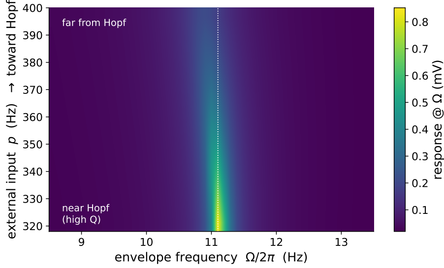
Figure S6: The resonance ridge sharpens and intensifies toward the Hopf (Jansen–Rit). De-modulated response A_\Omega over the (envelope frequency, input p ) plane. The ridge at f_0 \approx 11.1 Hz sharpens and intensifies as p approaches the Hopf from above, visualizing the 1/\gamma gain of Eq. (11).
