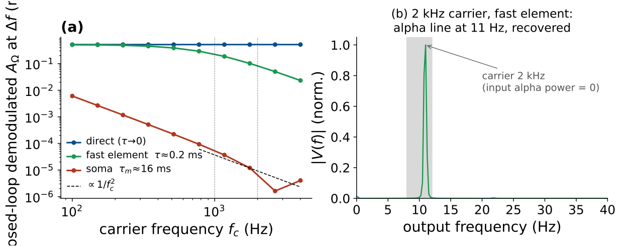
Figure S12: Demodulation at a genuine kHz carrier (Jansen–Rit, closed loop). The applied field passes through an explicit membrane filter before the sigmoid. (a) Closed-loop demodulated A_\Omega at \Delta f = f_0 vs. carrier f_c for three coupling routes: direct ( \tau \rightarrow 0 , carrier-independent), fast element (axon/AIS/node, \tau \approx 0.2 ms; survives into the kHz band), and soma ( \tau_m \approx 16 ms; collapses as 1/f_c^2 ). (b) Output spectrum for a 2 kHz carrier delivered through the fast element: a clean alpha line at f_0 , synthesized by the column although the input carries no alpha power.
