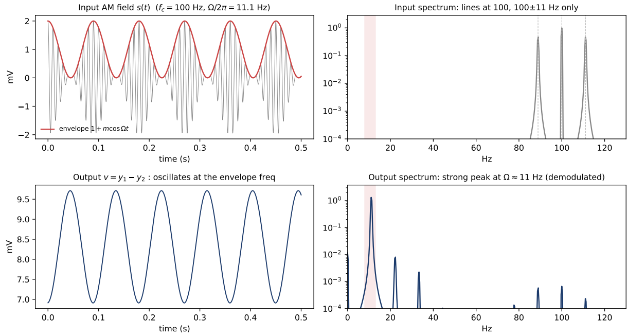
Figure 7: Demodulation in the Jansen–Rit column (proof of concept). Top left: the AM field s(t) and its envelope. Top right: the input spectrum has lines only at f_c and f_c \pm \Delta f (89, 100, 111 Hz); the alpha band (shaded) is empty. Bottom left: the output v = y_1 - y_2 oscillates at the envelope frequency. Bottom right: the output spectrum has a strong peak at \Omega \approx 11 Hz, synthesized by the sigmoid and absent from the input.
