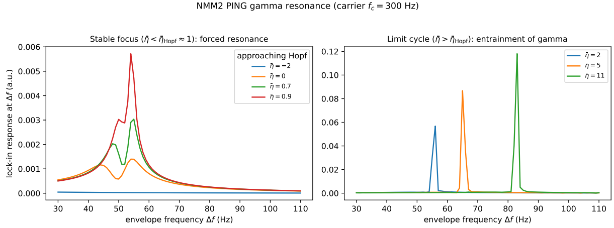
Figure 15: NMM2 PING gamma resonance (exact mean field). Lock-in response of the excitatory rate r_E at the envelope frequency \Delta f under an AM field (carrier 300 Hz). Left (stable focus, \bar{\eta} < \bar{\eta}_{\text{Hopf}} \approx 1 ): forced resonance at the gamma frequency ( f_0 \approx 55 Hz), growing as the Hopf is approached ( 1/\gamma gain), with the resonant frequency rising with \bar{\eta} . Right (limit cycle, \bar{\eta} > \bar{\eta}_{\text{Hopf}} ): entrainment of the autonomous gamma. The input carries no power at \Delta f ; the response is synthesized by the exact quadratic v^2 nonlinearity.
