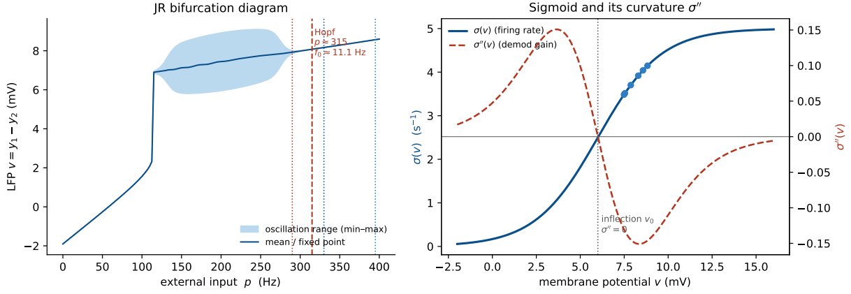
Figure 5: The Jansen–Rit operating regime: bifurcation and sigmoid curvature. Left: JR bifurcation diagram—LFP range vs. external input p . A limit cycle (alpha) exists between a saddle-node-on-invariant-circle (SNIC) bifurcation near p \approx 115 and the supercritical Hopf at p \approx 315 ; above the Hopf the fixed point is a stable focus, f_0 \approx 11.1 Hz. Right: the sigmoid \sigma(v) and its curvature \sigma''(v) , which sets the demodulation gain and vanishes at the inflection v_0 . Dots mark the operating points reached by the closed-loop model for the p values used here.
