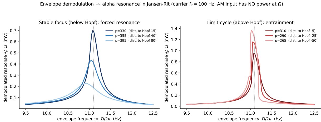
Figure 8: Resonance near vs. far from the Hopf (Jansen–Rit). Lock-in response at \Omega vs. envelope frequency ( \varepsilon = 0.3 mV). Left (stable focus, p > 315 ): forced resonance at f_0 \approx 11.1 Hz; the peak grows monotonically as p \rightarrow 315 , i.e. \text{gain} \propto 1/\gamma . Right (limit cycle, p < 315 ): the demodulated drive entrains the autonomous alpha rhythm.
