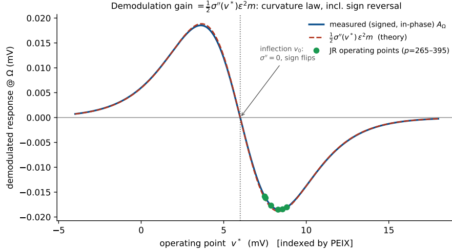
Figure 3: Operating-point law and the \sigma'' control (Jansen–Rit). The measured signed (in-phase) open-loop response tracks \frac{1}{2}\sigma''(v^*)\varepsilon^2 m across the whole range, vanishes at the inflection v_0 , and reverses sign across it—a direct verification that demodulation is the sigmoid-curvature term of Eq. (10). The closed-loop JR operating points (dots) sit on the lobe where \sigma'' is large and negative.
