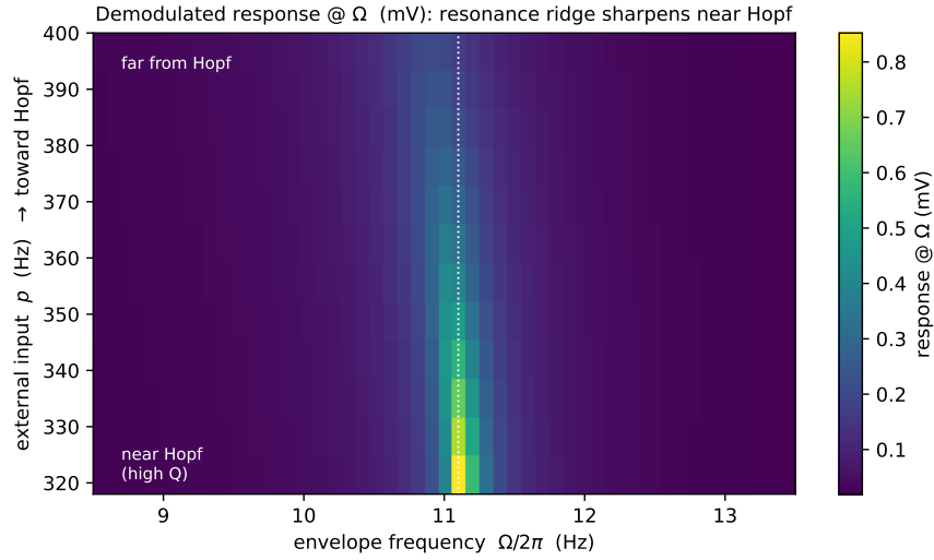
Figure 9: Resonance map (Jansen–Rit). Demodulated response A_\Omega over the (envelope frequency, input p ) plane. The ridge at f_0 \approx 11.1 Hz sharpens and intensifies as p approaches the Hopf from above, visualizing the 1/\gamma gain of Eq. (11).
