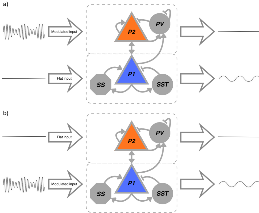
Figure 6: Stimulation setup in a LaNMM column. The column couples a superficial PING subcircuit (pyramidal P_2 + PV; gamma) and a deep JR subcircuit (pyramidal P_1 + SS + SST; alpha). (a) the AM input drives P_2 while P_1 receives a flat drive; (b) the AM input drives P_1 while P_2 is flat. Through the sigmoid nonlinearities and P_1 – P_2 coupling, the slow envelope is transferred to the column: P_2 carries the modulated fast carrier, while P_1 exposes the recovered low-frequency envelope (right traces).
