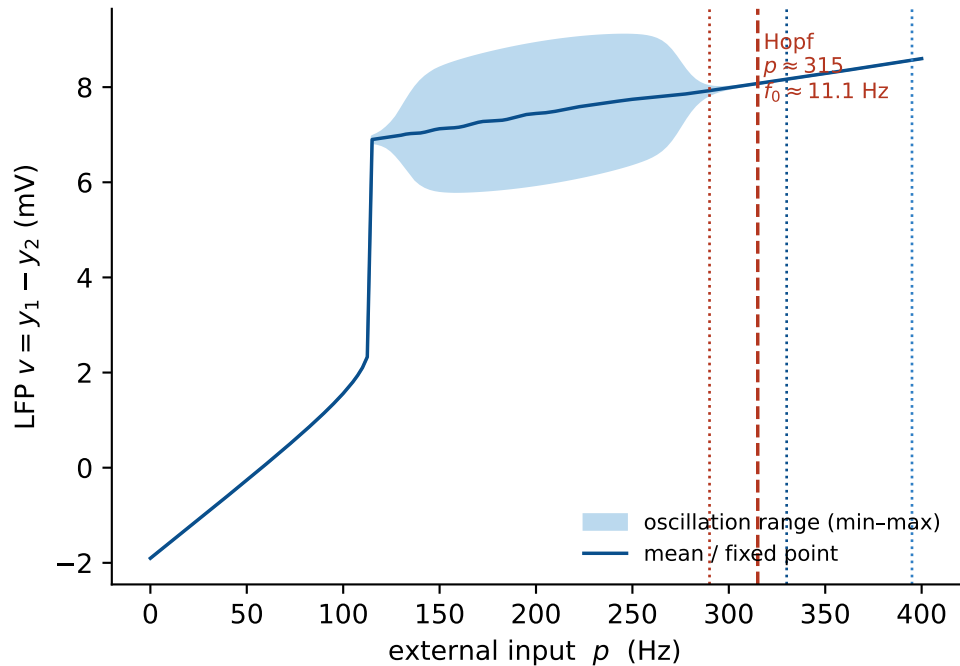
JR bifurcation diagram
