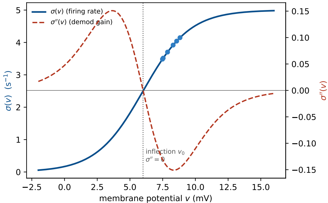
Sigmoid and its curvature \sigma''
