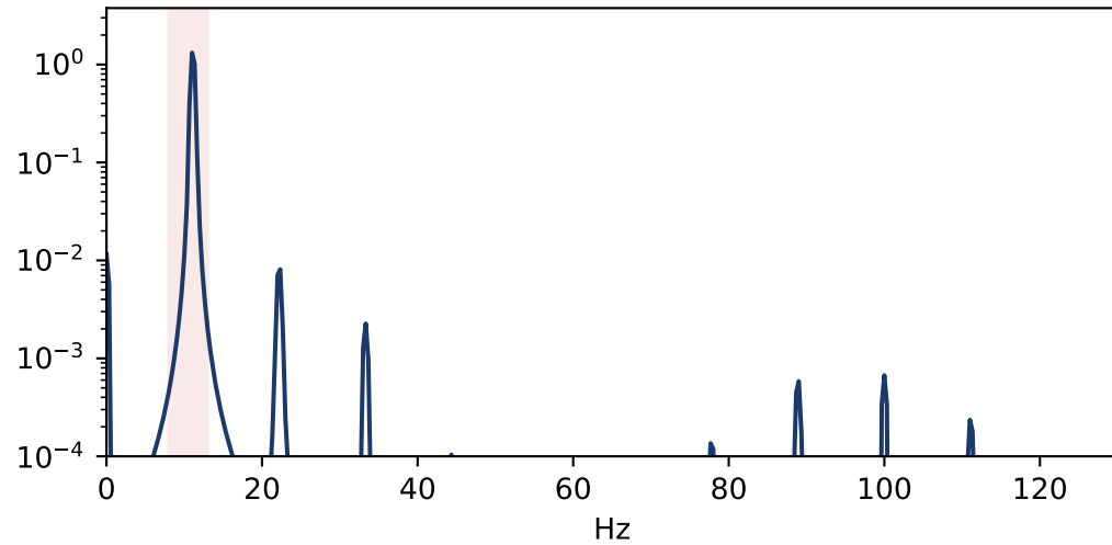
Output spectrum: strong peak at \Omega \approx 11 Hz (demodulated)
