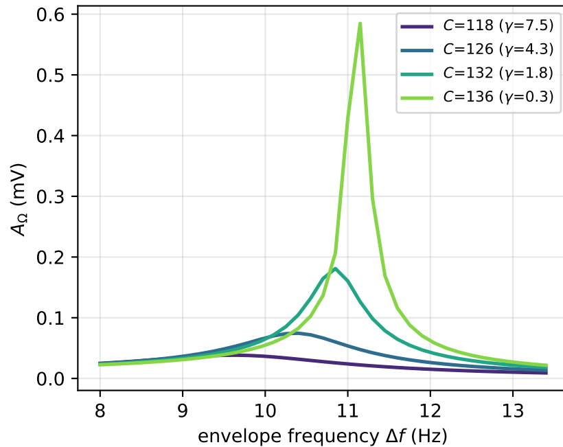
(b) resonance sharpens as C \rightarrow C^*
