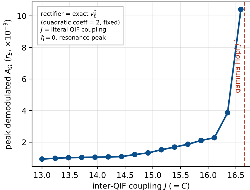
(a) NMM2 J curve (exact mean field)
