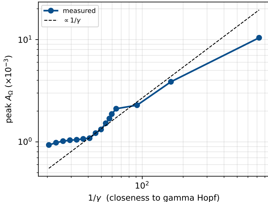
(b) amplification \propto 1/\gamma , saturating
