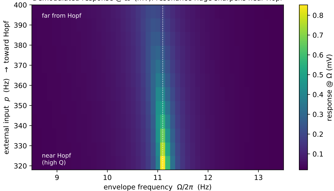
Demodulated response @ \Omega (mV): resonance ridge sharpens near Hopf
