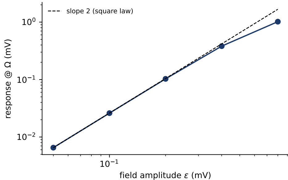
Square-law demodulation (response \propto \varepsilon^2 at small drive)
