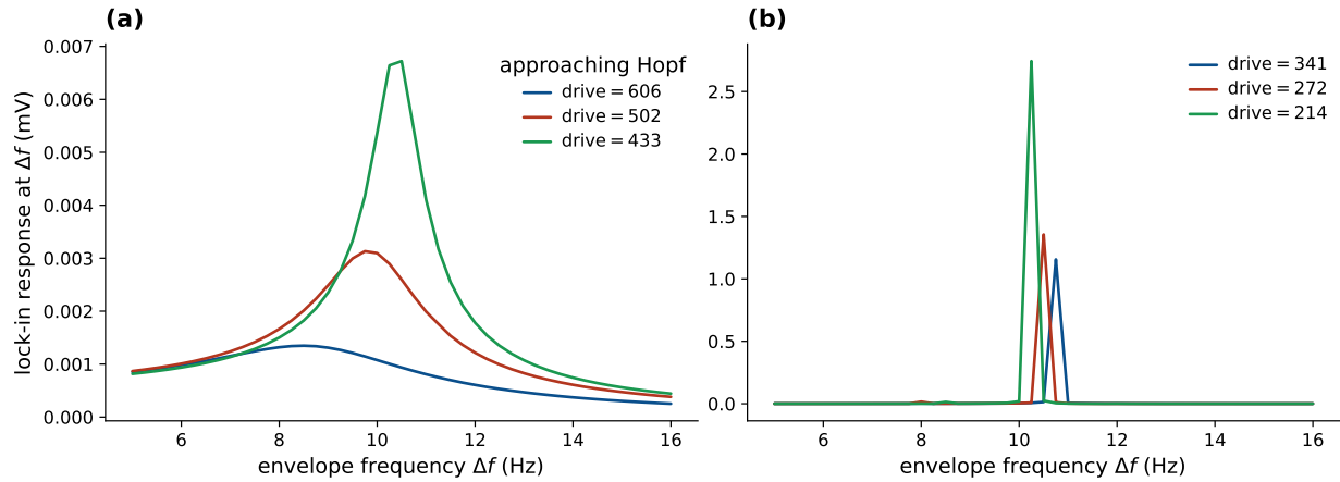
Figure S9: LaNMM alpha resonance (NMM1, laminar). Lock-in response of the deep pyramidal P_1 at the envelope frequency \Delta f , the P_1 (alpha) loop driven by an AM field (carrier 100 Hz) with its input as bifurcation parameter. (a) (stable focus, high drive) forced alpha resonance at \sim 10 Hz growing as the Hopf is approached. (b) (limit cycle, low drive) entrainment of the autonomous alpha. Directly parallel to the JR single column (Fig. 4).
