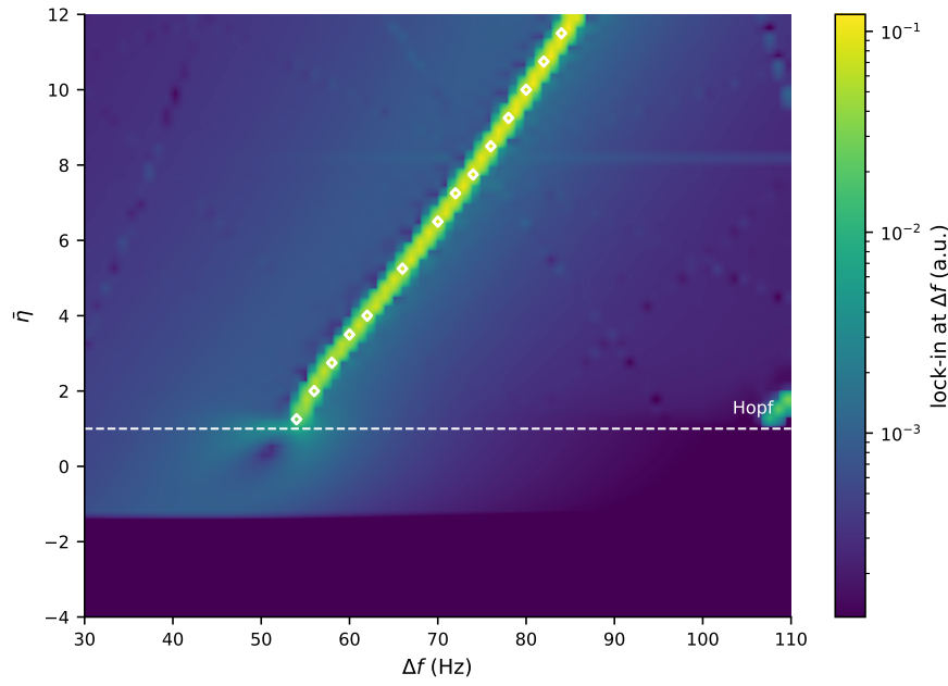
Figure S11: NMM2 PING resonance map (exact mean field). Demodulated response over the (envelope frequency \Delta f , background drive \bar{\eta} ) plane, log color scale. The ridge follows the gamma natural frequency f_0(\bar{\eta}) , and its diagonal slope, f_0 rising with \bar{\eta} , reflects the state-dependent transfer of NMM2, absent in the static-sigmoid JR and LaNMM. White markers outline the 1:1 frequency-captured set, |f_{\text{out}} - \Delta f| < 0.3 Hz (Appendix C), evaluated only above the Hopf (dashed line) where there is an autonomous rhythm to capture: entrainment tracks the ridge there, while the same color field below the Hopf is a forced response. Lock-in amplitude alone cannot separate the two, since both place power at \Delta f , which is why the locked set is drawn explicitly rather than inferred from the color.
