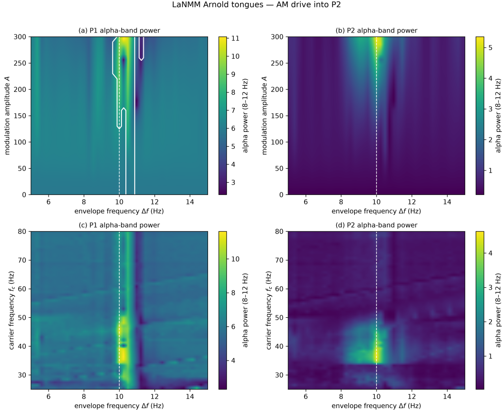
Figure 7: LaNMM Arnold tongues: AM input to the superficial P_2 (gamma) loop. (a,b) Alpha-band power of P_1 and P_2 vs. modulation amplitude A and beat frequency \Delta f (carrier 40 Hz), with elevated power around the P_1 alpha ( \sim 10 Hz, dashed line). White contour in (a): the 1:1 frequency-captured set, |f_{\text{out}} - \Delta f| < 0.3 Hz (Appendix C), which is what defines the tongue. Band power alone cannot separate capture from a forced response, since both place power at \Delta f ; the captured set is therefore computed from the dominant output frequency and drawn explicitly. Its width grows monotonically with drive, from \approx 0.6 Hz at A \rightarrow 0 (the tolerance-limited tip, 2 \times 0.3 = 0.6 Hz) to 1.75 Hz at A = 300 . (c,d) Alpha power vs. carrier frequency and \Delta f at A = 250 : P_1 demodulation requires both a carrier \approx 40 Hz ( P_2 gamma) and \Delta f \approx 10 Hz ( P_1 alpha)—a double resonance.
