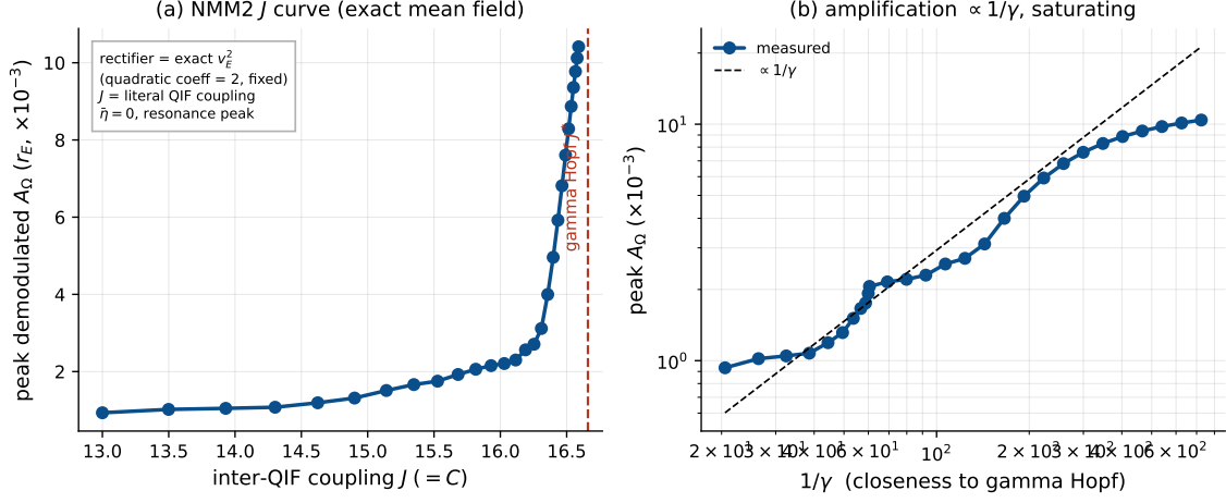
Figure S13: Coupling controls the amplification in the exact mean field (NMM2 PING, \gamma ). J ( = C ) is the literal inter-QIF synaptic weight; the rectifier is the exact v_E^2 (fixed quadratic coefficient), so no operating-point pinning is needed. (a) The peak demodulated response of r_E grows as J \rightarrow J^* (gamma Hopf, \bar{\eta} = 0 ; stable focus, \gamma > 0 ). (b) The gain grows as 1/\gamma (dashed), saturating near criticality—the JR law, now with coupling and rectifier both derived.
