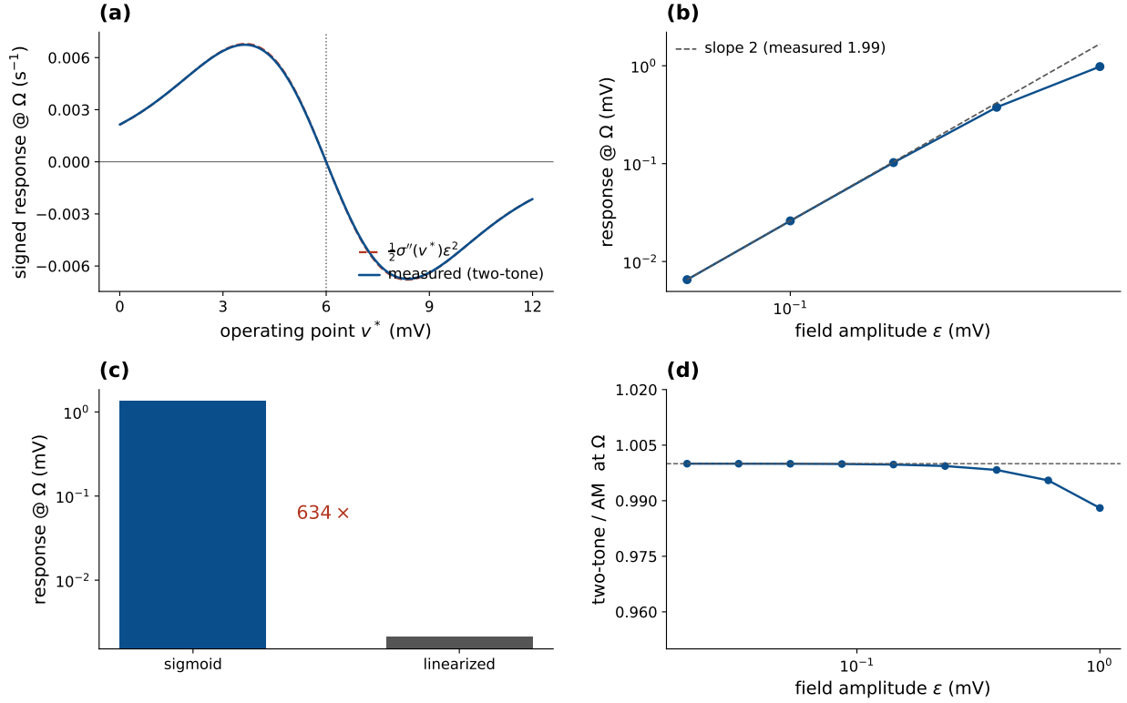
Figure 6: The curvature law, the square law, and the surrogate control (Jansen–Rit, genuine two tones). (a) The measured signed (in-phase) open-loop response tracks \frac{1}{2}\sigma''(v^*)\varepsilon^2 across the whole operating range (maximum deviation 0.9%), vanishes at the inflection v_0 , and reverses sign across it—a direct verification that demodulation is the sigmoid-curvature term of Eq. (10). The mechanism is sign-agnostic: \sigma'' sets the sign and phase of the demodulated response while |\sigma''| sets its gain, so the resonance picture is unchanged up to an overall sign in the \sigma'' > 0 lobe, which this sweep already spans. The sign flip is a falsifiable prediction (§4.10). (b) The closed-loop response scales as \varepsilon^2 at small drive, measured log–log slope 1.99 against the predicted 2. (c) Replacing the field-receiving sigmoid by its tangent at v^* collapses the response 634\times ( 1.34 \rightarrow 0.0021 mV): the nonlinearity is the detector. (d) Surrogate control. The ratio of the two-tone to the matched AM response at \Omega approaches 1 as \varepsilon \rightarrow 0 (1.0000 at 0.02 mV, 0.988 at 1 mV), confirming that the two waveforms agree on the leading \Omega component in the perturbative regime. This licenses the AM surrogate for the dense sweeps of Figs. 4 and 9, which measure only that component; it does not license it for DC or harmonic claims (§2.2).
