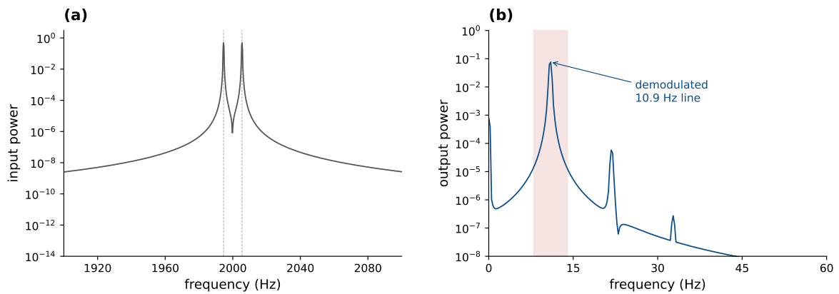
Figure S8: Genuine two-tone TI at a real kHz carrier (Jansen–Rit, fast-element route). Two equal tones at f_1 = 1994.5 and f_2 = 2005.5 Hz, beating at 10.9 Hz, pass through the fast-element low-pass ( \tau = 0.2 ms) into the recurrent column. (a) The input spectrum has lines only at f_1 and f_2 ; power in the 8–14 Hz band is 2.2 \times 10^{-13} , zero to numerical precision. (b) The output carries a clean demodulated line at 11.0 Hz. This is the kHz claim on the physical waveform rather than on the AM surrogate.
