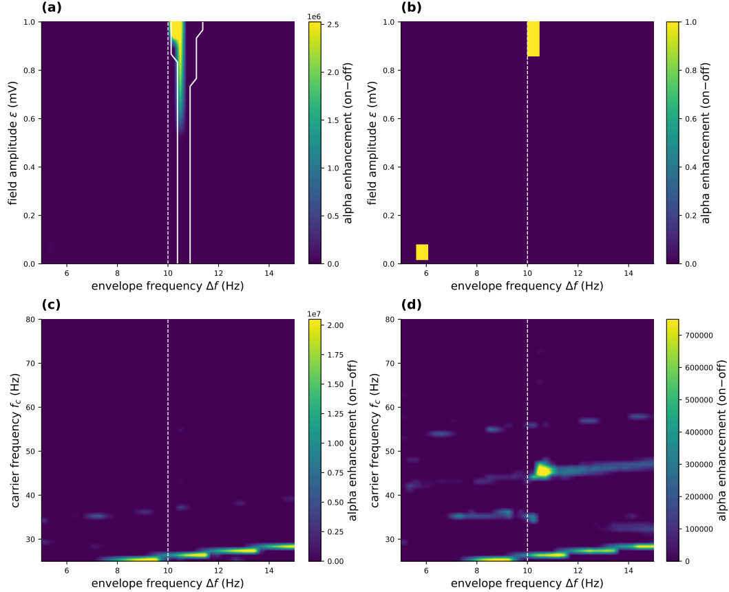
Figure S10: LaNMM Arnold tongues: two-tone TI field delivered directly to the deep P_1 (alpha) loop. As Fig. 7 but with the field on P_1 . The deep loop is captured by a much weaker field than the superficial one, so the amplitude range is \varepsilon \leq 1 mV here against 3 mV there; above \approx 2 mV the drive captures essentially the whole \Delta f sweep and leaves the perturbative regime the theory describes. Colour: stimulation-induced alpha-band enhancement over the \varepsilon = 0 baseline. (a,b) P_1 and P_2 enhancement vs. \varepsilon and \Delta f ; the white contour in (a) outlines the 1:1 frequency-captured set, |f_{\text{out}} - \Delta f| < 0.3 Hz (Appendix C), computed from the dominant output frequency because band power alone cannot separate capture from a forced response. Its width grows from 0.5 Hz at \varepsilon \rightarrow 0 to 1.25 Hz at \varepsilon = 1 mV. (c,d) Enhancement vs. carrier frequency and \Delta f at \varepsilon = 0.5 mV. P_1 responds across a broad carrier band—a vertical ridge at \Delta f \approx 10 Hz, the direct-coupling limit of Eq. (10). Read with the lock-in at \Delta f the response is retained at every carrier from 25 to 80 Hz (median 25% of peak), in contrast to the \sim 7\% collapse off resonance under superficial drive.
