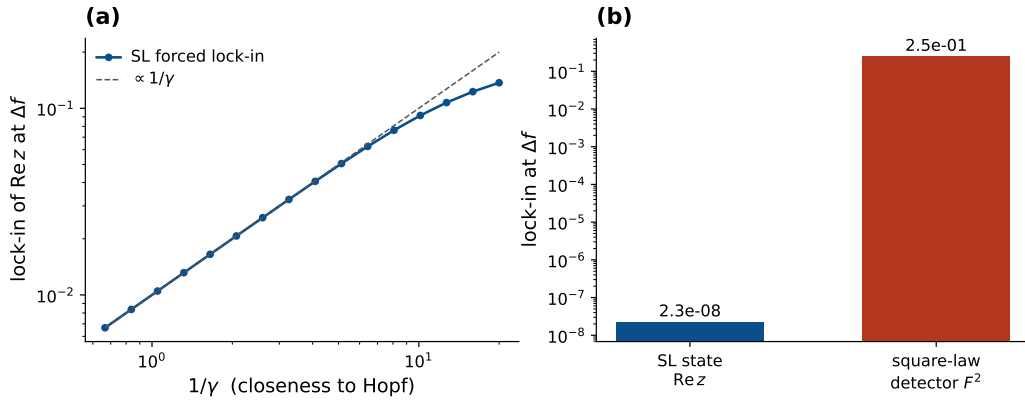
Figure S1: Stuart–Landau dissociation: amplification without detection. SL normal form (Eq. (22)). (a) Driven directly in band at \Delta f (tACS-like; weak drive, linear regime), the forced lock-in of \text{Re } z grows as 1/\gamma toward the Hopf—the universal near-Hopf amplification. (b) Under the AM carrier (TI), the \Delta f line in \text{Re } z sits at the numerical floor ( \sim 2 \times 10^{-8} ), while a square-law detector F^2 recovers it ( 2.5 \times 10^{-1} )—a \sim 10^7 \times gap. The normal form amplifies but cannot demodulate.
