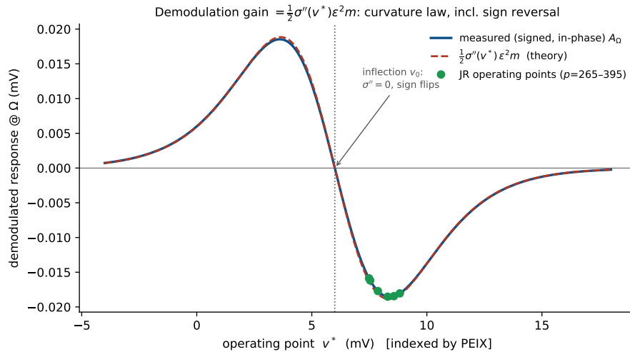
Figure 9: Operating-point law and the \sigma'' control (Jansen–Rit). The measured signed (in-phase) open-loop response tracks \frac{1}{2}\sigma''(v^*)\varepsilon^2 m across the whole range, vanishes at the inflection v_0 , and reverses sign across it—a direct verification that demodulation is the sigmoid-curvature term of Eq. (10). The closed-loop JR operating points (dots) sit on the lobe where \sigma'' is large and negative.
