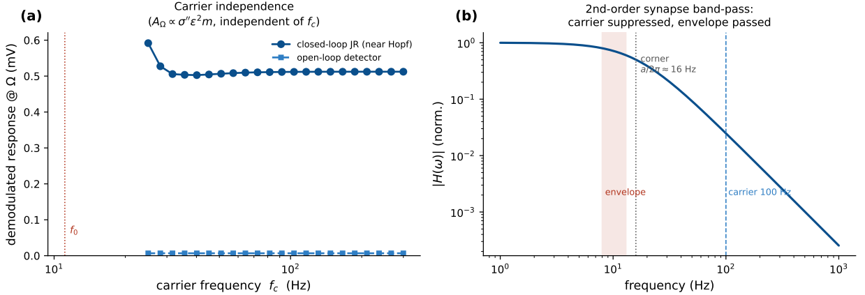
Figure 5: The demodulated response is carrier-independent at fixed polarization (Jansen–Rit). Left: the demodulated response is flat across carrier frequency f_c = 25 – 300 Hz, both for the open-loop detector (exactly, by Eq. (10)) and for the closed-loop JR near the Hopf (which adds \sim 60\times resonant gain); deviations appear only as f_c approaches the natural band. Right: the second-order-synapse band-pass |H(\omega)| passes the envelope ( \sim 0.7 ) and suppresses the 100 Hz carrier ( \sim 2.5\% ).
