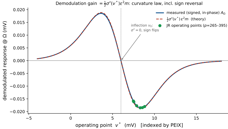
Figure 7: Operating-point law and the \sigma'' control (Jansen–Rit). The measured signed (in-phase) open-loop response tracks \frac{1}{2}\sigma''(v^*)\epsilon^2 m across the whole range, vanishes at the inflection v_0 , and reverses sign across it—a direct verification that demodulation is the sigmoid-curvature term of Eq. (10). The closed-loop JR operating points (dots) sit on the lobe where \sigma'' is large and negative—not by design, but because that is where the JR resting point lies as the alpha Hopf is approached (the saturating upper flank of the sigmoid). The mechanism is sign-agnostic: \sigma'' sets only the sign/phase of the demodulated response while |\sigma''| sets its gain, so the entire resonance picture is unchanged (up to an overall sign) in the \sigma'' > 0 lobe, which this open-loop sweep already spans. The sign flip itself is a falsifiable prediction (§4.10).
