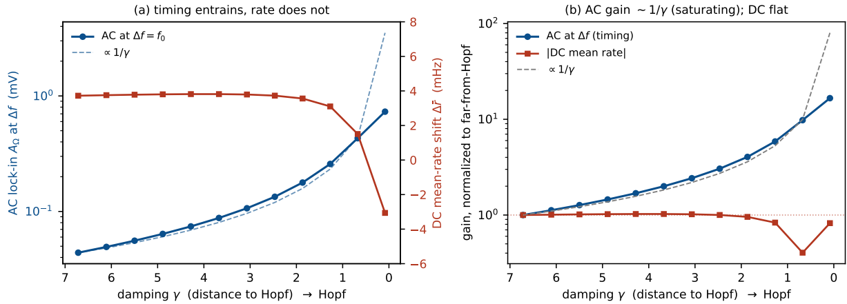
Figure 18: Timing, not rate (Jansen-Rit, detection pinned). As the column is driven toward the Hopf through the coupling at fixed \sigma''(v^*) , (a) the AC lock-in at the resonant beat \Delta f = f_0 (blue) is resonantly amplified and tracks 1/\gamma (dashed), while the DC shift of the mean firing rate (red) stays flat at a few mHz. (b) Normalized to the far-from-Hopf value (log scale): the AC gain follows 1/\gamma and saturates near criticality, whereas the DC gain stays \sim 1 . The envelope entrains timing, not rate—the population analog of the spike-timing-without-rate finding of [6].
