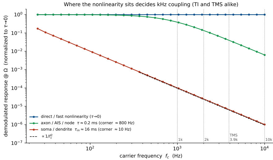
Figure 7: Carrier frequency in the kHz regime (Jansen–Rit, open-loop detector). Open-loop demodulated response (normalized to the \tau \rightarrow 0 value) vs. carrier frequency up to 10 kHz. With direct coupling ( \tau \rightarrow 0 ) the response is flat—carrier-independent. A slow somatic membrane ( \tau_m \approx 16 ms) rolls off as 1/f_c^2 (dashed guide), killing kHz demodulation; a fast element (axon/AIS/node, \tau \approx 0.2 ms) retains an appreciable response into the kHz band ( \sim 0.14 at 2 kHz, \sim 0.04 at the TMS peak 3.9 kHz). The same membrane filter attenuates TMS at the soma, which is why neither TMS nor TI should be thought of as driving the soma at kHz.
