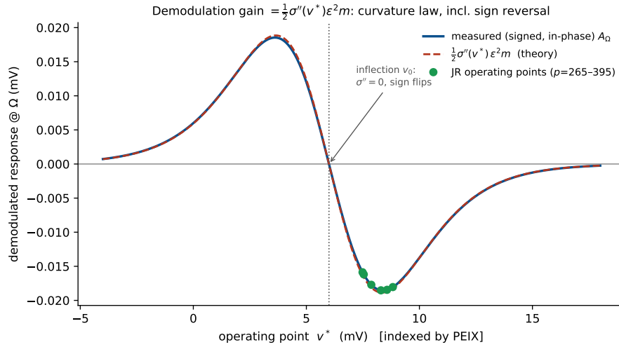
Figure 9: Operating-point law and the \sigma'' control (Jansen–Rit). The measured signed (in-phase) open-loop response tracks \frac{1}{2}\sigma''(v^*)\epsilon^2 m across the whole range, vanishes at the inflection v_0 , and reverses sign across it—a direct verification that demodulation is the sigmoid-curvature term of Eq. (10). The closed-loop JR operating points (dots) sit on the lobe where \sigma'' is large and negative.
