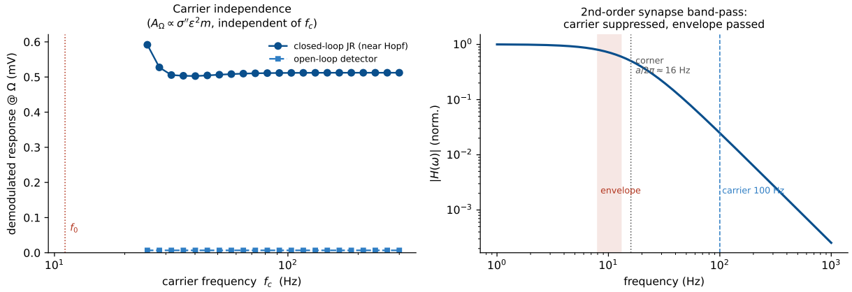
Figure 6: Carrier independence (Jansen–Rit single column). Left: the demodulated response is flat across carrier frequency f_c = 25\text{--}300 Hz, both for the open-loop detector (exactly, by Eq. (10)) and for the closed-loop JR near the Hopf (which adds \sim 60\times resonant gain); deviations appear only as f_c approaches the natural band. Right: the second-order-synapse band-pass |H(\omega)| passes the envelope ( \sim 0.7 ) and suppresses the 100 Hz carrier ( \sim 2.5\% ).
