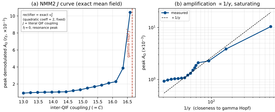
Figure 17: Coupling controls the amplification in the exact mean field (NMM2 PING, gamma). J (= C) is the literal inter-QIF synaptic weight; the rectifier is the exact v_E^2 (fixed quadratic coefficient), so no operating-point pinning is needed. (a) The peak demodulated response of r_E diverges as J \rightarrow J^* (gamma Hopf, \bar{\eta} = 0 ). (b) The gain grows as 1/\gamma (dashed), saturating near criticality—the JR law, now with coupling and rectifier both derived.
