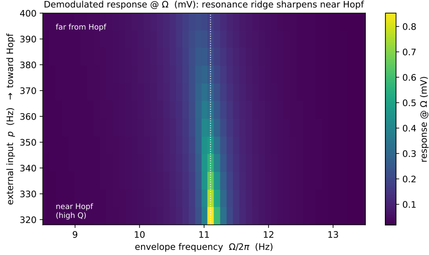
Figure 5: Resonance map (Jansen–Rit). Demodulated response A_\Omega over the (envelope frequency, input p ) plane. The ridge at f_0 \approx 11.1 Hz sharpens and intensifies as p approaches the Hopf from above, visualizing the 1/\gamma gain of Eq. (11).
