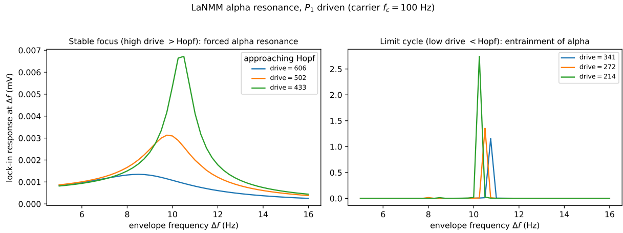
Figure 11: LaNMM alpha resonance (NMM1, laminar). Lock-in response of the deep pyramidal P_1 at the envelope frequency \Delta f , the P_1 (alpha) loop driven by an AM field (carrier 100 Hz) with its input as bifurcation parameter. Left (stable focus, high drive): forced alpha resonance at \sim 10 Hz growing as the Hopf is approached. Right (limit cycle, low drive): entrainment of the autonomous alpha. Directly parallel to the JR single column (Fig. 4).
