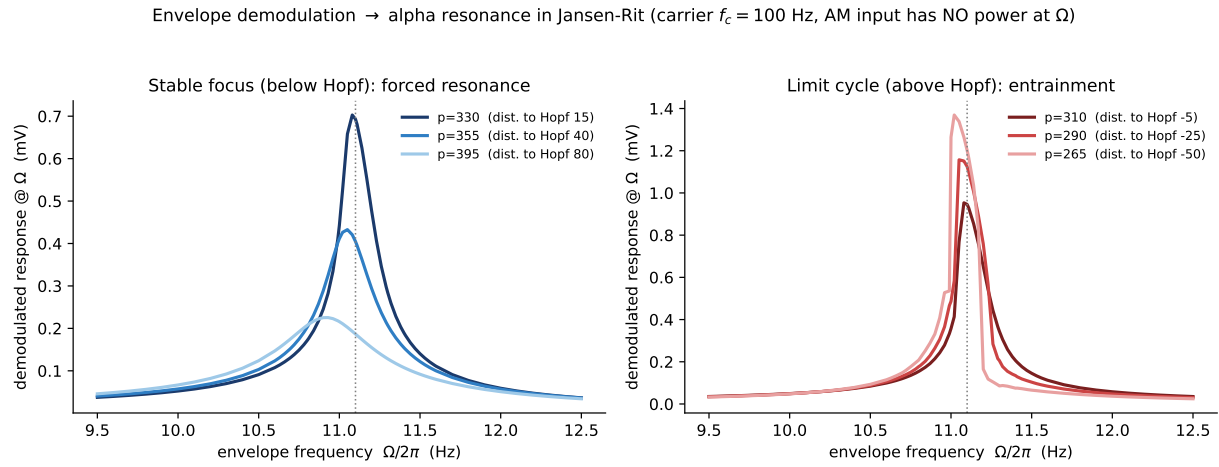
Figure 4: Resonance near vs. far from the Hopf (Jansen–Rit). Lock-in response at \Omega vs. envelope frequency ( \varepsilon = 0.3 mV). Left (stable focus, p > 315 ): forced resonance at f_0 \approx 11.1 Hz; the peak grows monotonically as p \rightarrow 315 , i.e. gain \propto 1/\gamma . Right (limit cycle, p < 315 ): the demodulated drive entrains the autonomous alpha rhythm.
