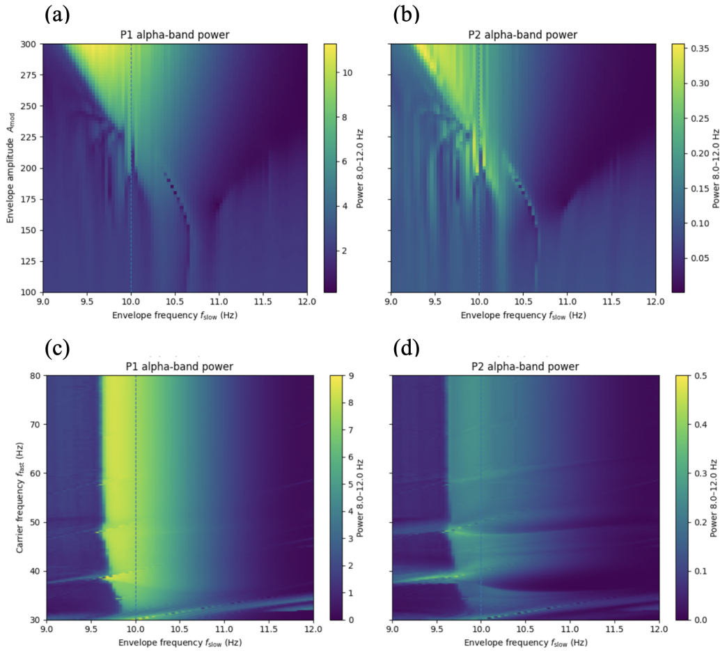
Figure 13: LaNMM Arnold tongues: AM input delivered directly to the deep P_1 (alpha) loop. (a,b) Alpha power of P_1 and P_2 vs. amplitude A and \Delta f . (c,d) Alpha power vs. carrier frequency and \Delta f : P_1 responds across a broad carrier band (a vertical ridge at \Delta f \approx 10 Hz)—carrier-independent, the direct-coupling limit of Eq. (10).
