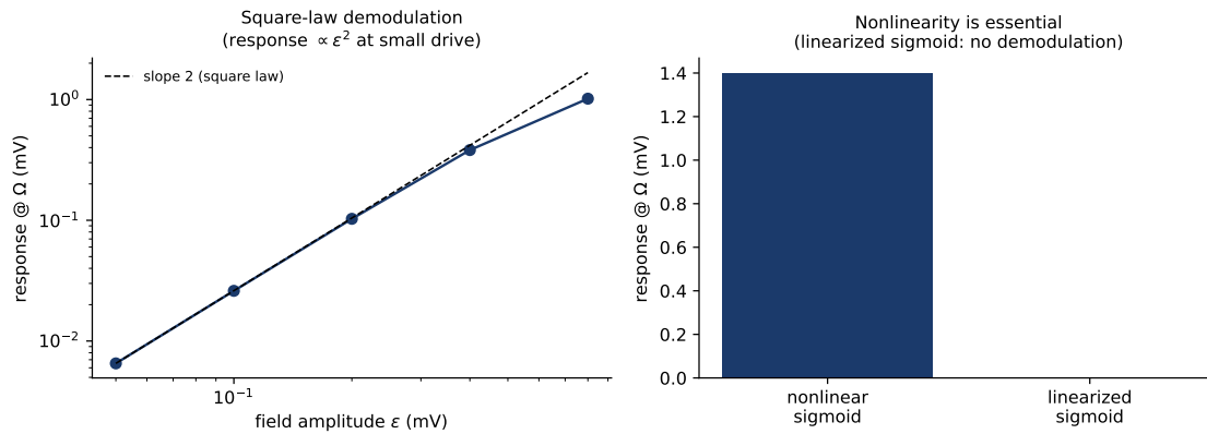
Figure 10: Verification (Jansen–Rit): square-law scaling and the linearization control. Left: response vs. field amplitude; small-drive log–log slope = 1.99 (theory 2). Right: linearizing the field-receiving sigmoid collapses the response 712\times ( 1.40 \rightarrow 0.0020 mV)—the nonlinearity is the demodulator.
