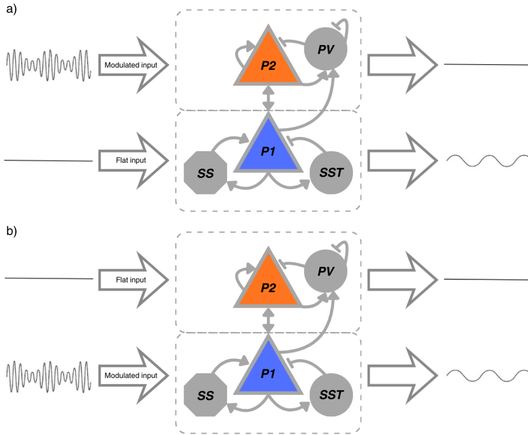
Figure S1: Stimulation setup in a LaNMM column. The column couples a superficial PING subcircuit (pyramidal P_2 + PV; gamma) and a deep JR subcircuit (pyramidal P_1 + SS + SST; alpha). (a) the AM input drives P_2 while P_1 receives a flat drive; (b) the AM input drives P_1 while P_2 is flat. Through the sigmoid nonlinearities and P_1 – P_2 coupling, the slow envelope is transferred to the column: P_2 carries the modulated fast carrier, while P_1 exposes the recovered low-frequency envelope (right traces).
