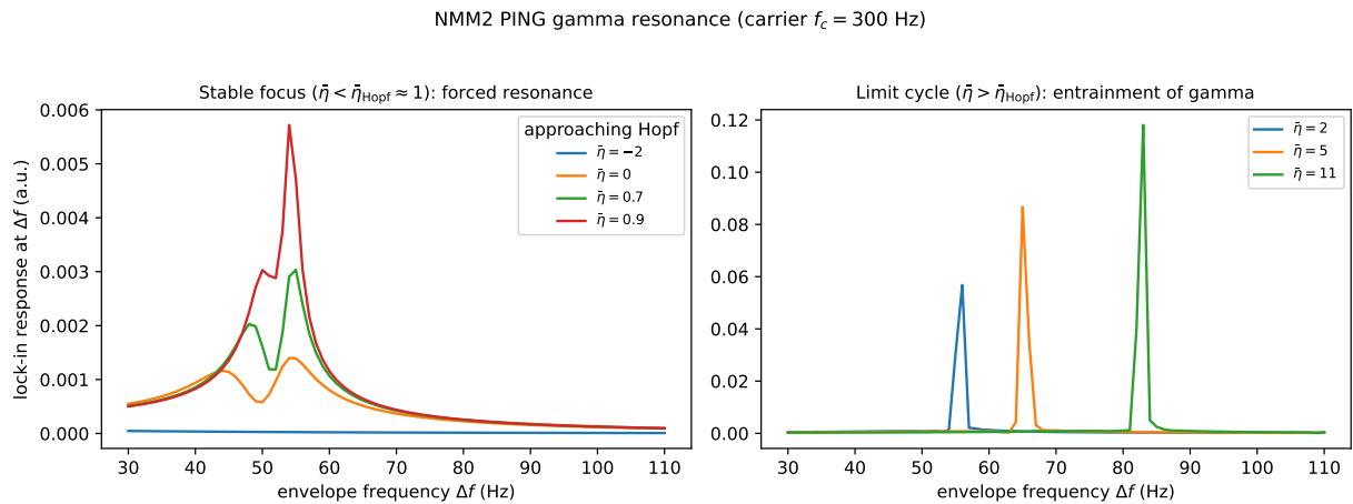
Figure 14: NMM2 PING gamma resonance (exact mean field). Lock-in response of the excitatory rate r_E at the envelope frequency \Delta f under an AM field (carrier 300 Hz). Left (stable focus, \tilde{\eta} < \tilde{\eta}_{\text{Hopf}} \approx 1 ): forced resonance at the gamma frequency ( f_0 \approx 55 Hz), growing as the Hopf is approached ( 1/\gamma gain), with the resonant frequency rising with \tilde{\eta} . Right (limit cycle, \tilde{\eta} > \tilde{\eta}_{\text{Hopf}} ): entrainment of the autonomous gamma. The input carries no power at \Delta f ; the response is synthesized by the exact quadratic v^2 nonlinearity.
