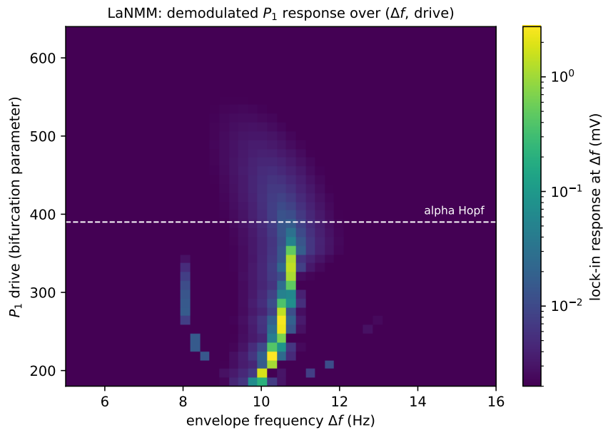
Figure S2: LaNMM alpha resonance map (NMM1, laminar). Demodulated P_1 response (log scale) over the (envelope frequency \Delta f , P_1 drive) plane: a ridge at the alpha natural frequency ( \sim 10 Hz) that intensifies through the supercritical Hopf (dashed line). The analog of the JR map (Fig. 5) and the NMM2 map (Fig. 15).
