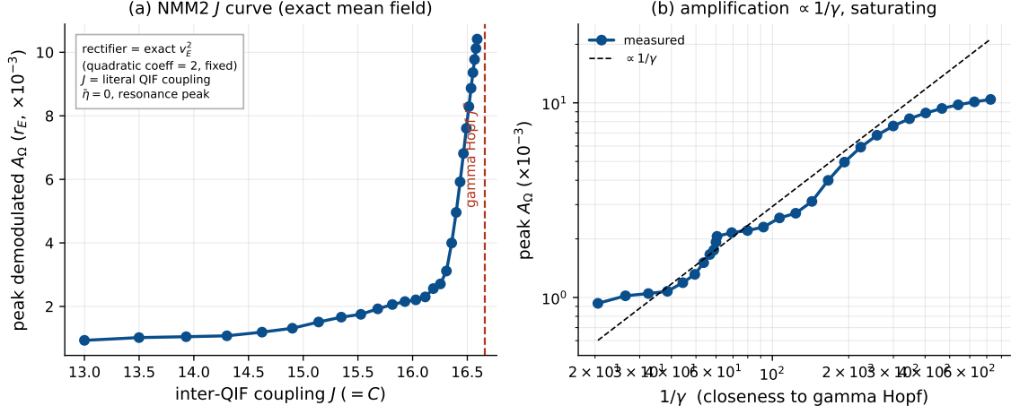
Figure 11: Coupling controls the amplification in the exact mean field (NMM2 PING, gamma). J (= C) is the literal inter-QIF synaptic weight; the rectifier is the exact v_E^2 (fixed quadratic coefficient), so no operating-point pinning is needed. (a) The peak demodulated response of r_E grows as J \rightarrow J^* (gamma Hopf, \bar{\eta} = 0 ; stable focus, \gamma > 0 ). (b) The gain grows as 1/\gamma (dashed), saturating near criticality—the JR law, now with coupling and rectifier both derived.
