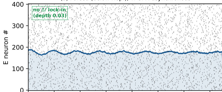
(a) Forced (below Hopf), TI OFF: asynchronous
