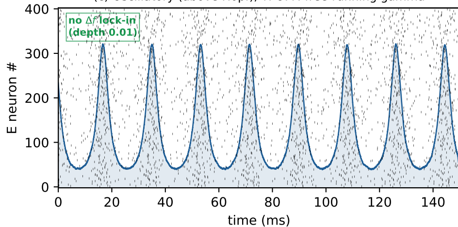
(c) Oscillatory (above Hopf), TI OFF: free-running gamma
