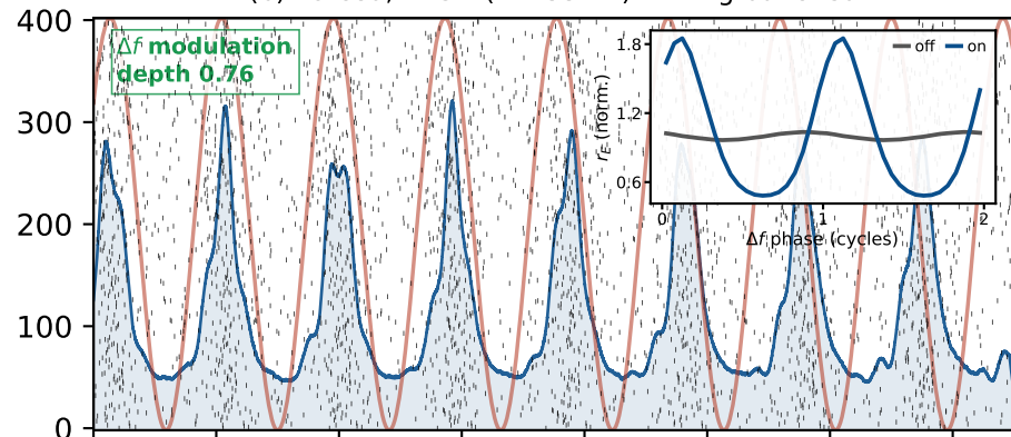
(b) Forced, TI ON ( \Delta f=55 Hz): timing bunched
