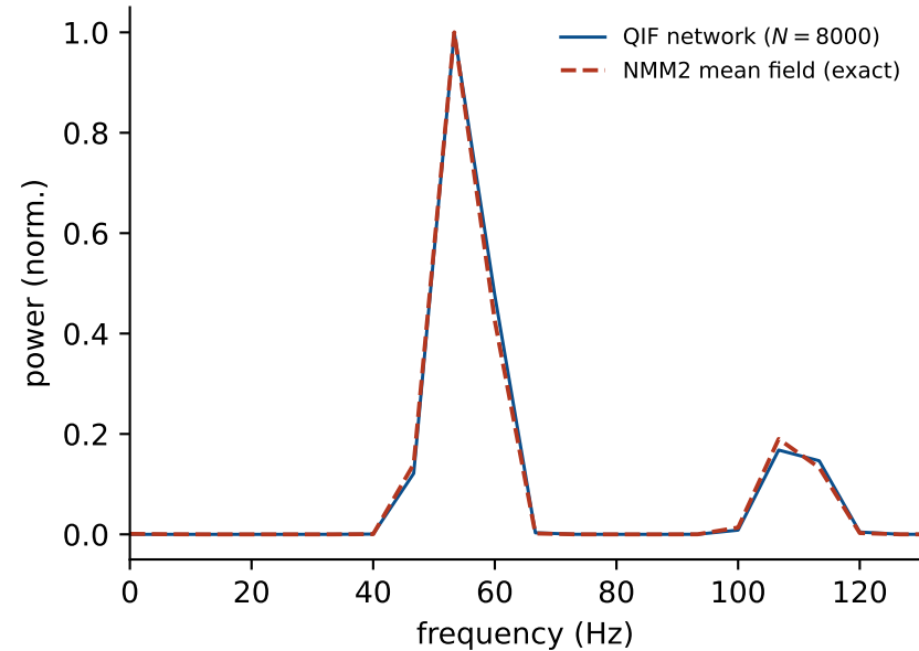
(a) QIF \rightarrow NMM2: matched autonomous gamma ( \langle r_E \rangle : 0.053 QIF vs 0.052 mean field)
