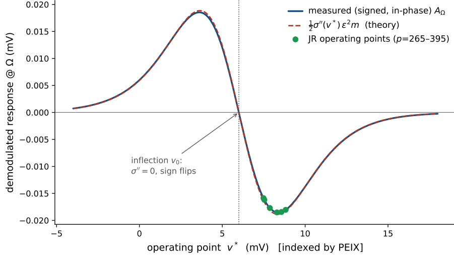
Figure 6: Operating-point law and the \sigma'' control (Jansen–Rit). The measured signed (in-phase) open-loop response tracks \frac{1}{2}\sigma''(v^*)\varepsilon^2 m across the whole range, vanishes at the inflection v_0 , and reverses sign across it—a direct verification that demodulation is the sigmoid-curvature term of Eq. (10). The closed-loop JR operating points (dots) sit on the lobe where \sigma'' is large and negative—not by design, but because that is where the JR resting point lies as the alpha Hopf is approached (the saturating upper flank of the sigmoid). The mechanism is sign-agnostic: \sigma'' sets only the sign/phase of the demodulated response while |\sigma''| sets its gain, so the entire resonance picture is unchanged (up to an overall sign) in the \sigma'' > 0 lobe, which this open-loop sweep already spans. The sign flip itself is a falsifiable prediction (§4.10).
