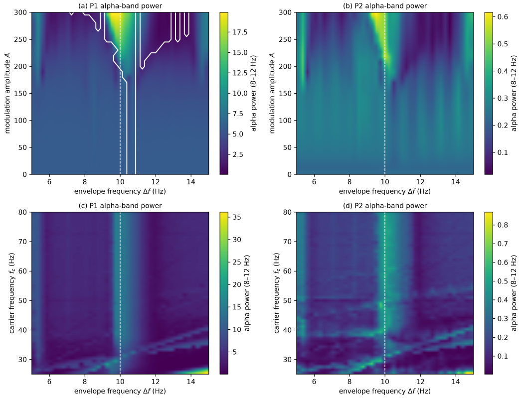
Figure S10: LaNMM Arnold tongues: AM input delivered directly to the deep P_1 (alpha) loop. (a,b) Alpha power of P_1 and P_2 vs. amplitude A and \Delta f ; the white contour in (a) outlines the 1:1 frequency-captured set, |f_{\text{out}} - \Delta f| < 0.3 Hz (Appendix C), computed from the dominant output frequency because band power alone cannot separate capture from a forced response. (c,d) Alpha power vs. carrier frequency and \Delta f : P_1 responds across a broad carrier band (a vertical ridge at \Delta f \approx 10 Hz)—carrier-independent, the direct-coupling limit of Eq. (10).
