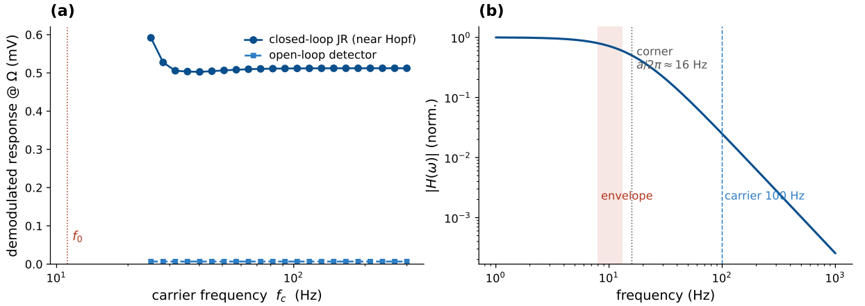
Figure 5: The demodulated response is carrier-independent at fixed polarization (Jansen–Rit). (a) The demodulated response is flat across carrier frequency f_c = 25 – 300 Hz, both for the open-loop detector (exactly, by Eq. (10)) and for the closed-loop JR near the Hopf (which adds \sim 60\times resonant gain); deviations appear only as f_c approaches the natural band. (b) The second-order-synapse band-pass |H(\omega)| passes the envelope ( \sim 0.7 ) and suppresses the 100 Hz carrier ( \sim 2.5\% ).
