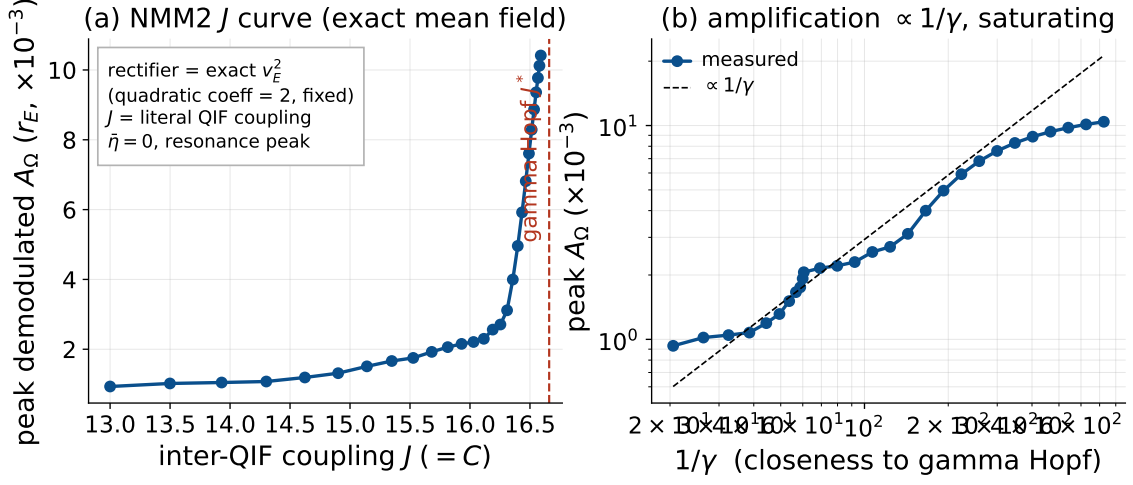
Figure S13: Coupling controls the amplification in the exact mean field (NMM2 PING, gamma). J(=C) is the literal inter-QIF synaptic weight; the rectifier is the exact v_E^2 (fixed quadratic coefficient), so no operating-point pinning is needed. (a) The peak demodulated response of r_E grows as J \rightarrow J^* (gamma Hopf, \bar{\eta} = 0 ; stable focus, \gamma > 0 ). (b) The gain grows as 1/\gamma (dashed), saturating near criticality—the JR law, now with coupling and rectifier both derived.
