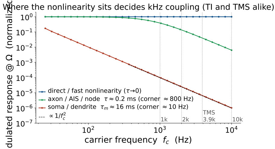
Figure S7: Somatic demodulation dies at kHz, but a fast element survives (Jansen–Rit, open-loop detector). Open-loop demodulated response (normalized to the \tau \rightarrow 0 value) vs. carrier frequency up to 10 kHz. With direct coupling ( \tau \rightarrow 0 ) the response is flat—carrier-independent. A slow somatic membrane ( \tau_m \approx 16 ms) rolls off as 1/f_c^2 (dashed guide), killing kHz demodulation; a fast element (axon/AIS/node, \tau \approx 0.2 ms) retains an appreciable response into the kHz band ( \sim 0.14 at 2 kHz, \sim 0.04 at the TMS peak 3.9 kHz). The same membrane filter attenuates TMS at the soma, which is why neither TMS nor TI should be thought of as driving the soma at kHz.
