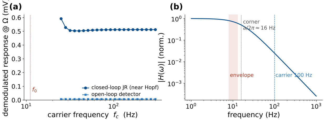
Figure 5: The demodulated response is carrier-independent at fixed polarization (Jansen–Rit). (a) The demodulated response is flat across carrier frequency f_c = 25 –300 Hz, both for the open-loop detector (exactly, by Eq. (10)) and for the closed-loop JR near the Hopf (which adds \sim 60\times resonant gain); deviations appear only as f_c approaches the natural band. (b) The second-order-synapse band-pass |H(\omega)| passes the envelope ( \sim 0.7 ) and suppresses the 100 Hz carrier ( \sim 2.5\% ).
