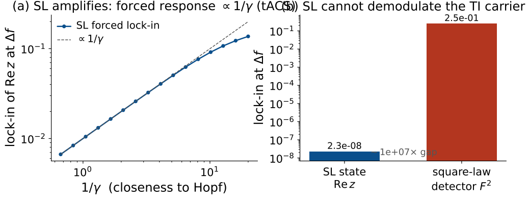
Figure S1: Stuart–Landau dissociation: amplification without detection. SL normal form (Eq. (17)). (a) Driven directly in band at \Delta f (tACS-like; weak drive, linear regime), the forced lock-in of \text{Re } z grows as 1/\gamma toward the Hopf—the universal near-Hopf amplification. (b) Under the AM carrier (TI), the \Delta f line in \text{Re } z sits at the numerical floor ( \sim 2 \times 10^{-8} ), while a square-law detector F^2 recovers it ( 2.5 \times 10^{-1} )—a \sim 10^7 \times gap. The normal form amplifies but cannot demodulate.
