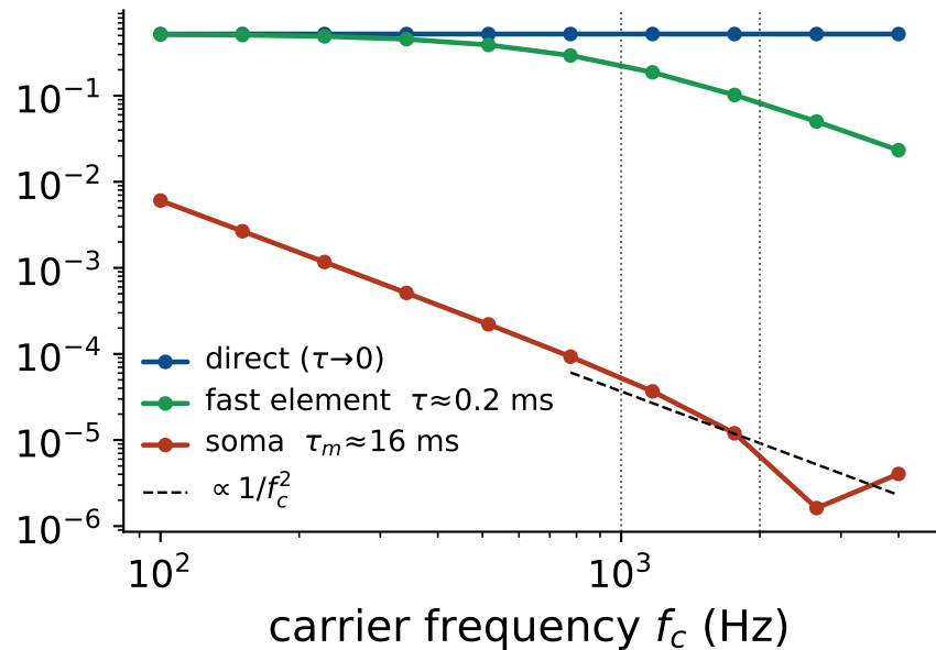
(a) the column demodulates into the kHz band via a fast element
