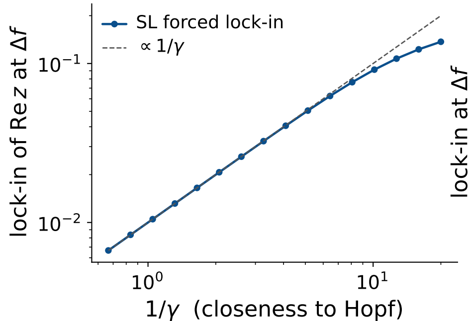
(a) SL amplifies: forced response \propto 1/\gamma (tAC)
