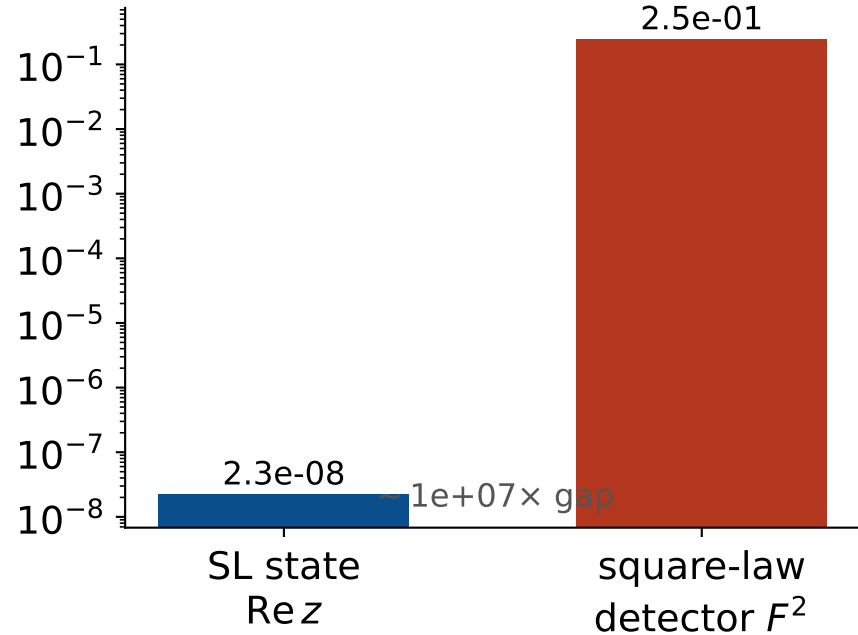
(b) SL cannot demodulate the TI carrier
