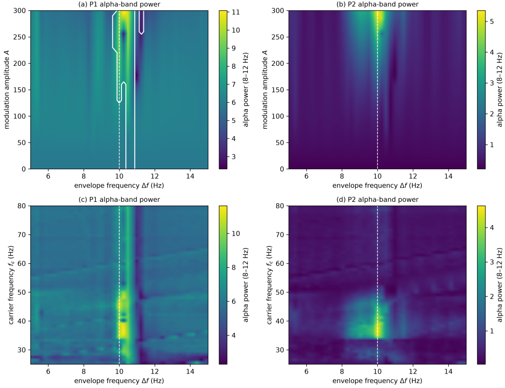
Figure 7: LaNMM Arnold tongues: AM input to the superficial P_2 (gamma) loop. (a, b) Alpha-band power of P_1 and P_2 vs. modulation amplitude A and beat frequency \Delta f (carrier 40 Hz), with elevated power around the P_1 alpha ( \sim 10 Hz, dashed line). White contour in (a) : the 1:1 frequency-captured set, |f_{\text{out}} - \Delta f| < 0.3 Hz (Appendix C), which is what defines the tongue. Band power alone cannot separate capture from a forced response, since both place power at \Delta f ; the captured set is therefore computed from the dominant output frequency and drawn explicitly. Its width grows monotonically with drive, from \approx 0.6 Hz at A \rightarrow 0 (the tolerance-limited tip, 2 \times 0.3 = 0.6 Hz) to 1.75 Hz at A = 300 . (c, d) Alpha power vs. carrier frequency and \Delta f at A = 250 : P_1 demodulation requires both a carrier \approx 40 Hz ( P_2 gamma) and \Delta f \approx 10 Hz ( P_1 alpha)—a double resonance.
