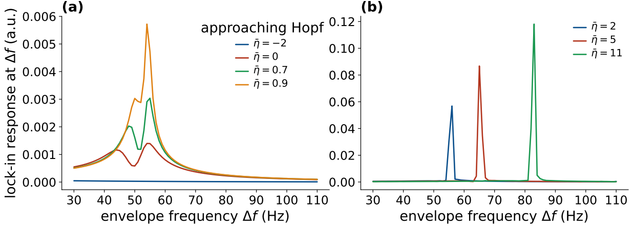
Figure 8: NMM2 PING gamma resonance (exact mean field). Lock-in response of the excitatory rate r_E at the envelope frequency \Delta f under an AM field (carrier 300 Hz). (a) (stable focus, \tilde{\eta} < \tilde{\eta}_{\text{Hopf}} \approx 1 ) forced resonance at the gamma frequency ( f_0 \approx 55 Hz), growing as the Hopf is approached ( 1/\gamma gain), with the resonant frequency rising with \tilde{\eta} . (b) (limit cycle, \tilde{\eta} > \tilde{\eta}_{\text{Hopf}} ) entrainment of the autonomous gamma. The input carries no power at \Delta f ; the response is synthesized by the exact quadratic v^2 nonlinearity.
