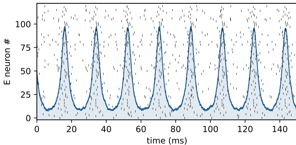
(c) Entrained (above Hopf), TI OFF: free gamma
