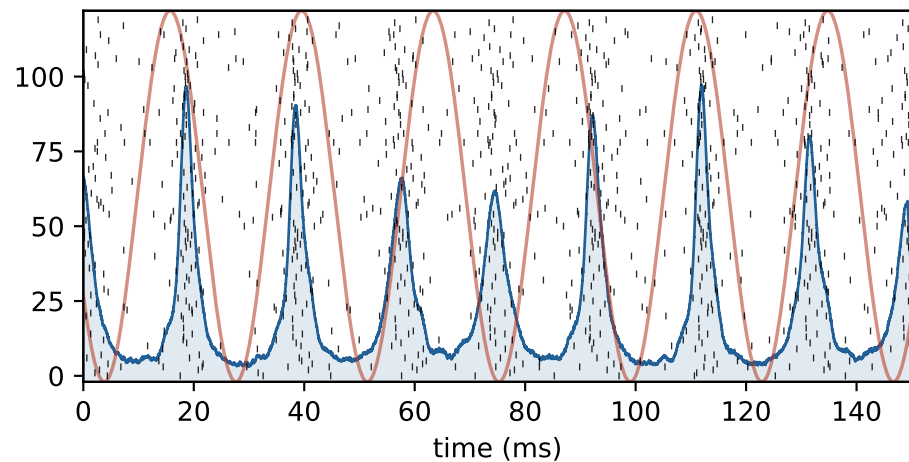
(d) Entrained, TI ON ( \Delta f=42 Hz): re-timed to TI
