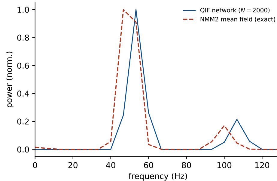
(a) QIF \rightarrow NMM2: matched gamma spectrum ( \langle r_E \rangle : 0.058 QIF vs 0.057 mean field)
