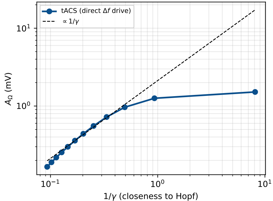
(b) same 1/\gamma amplification as TI
