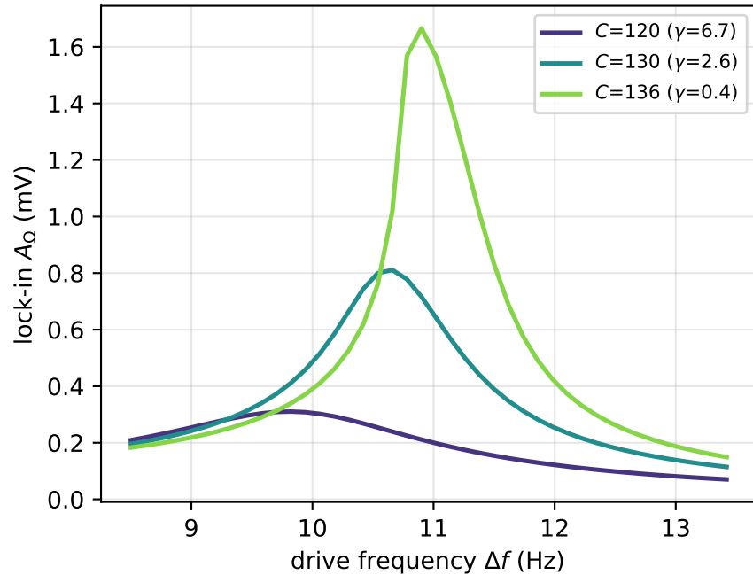
(a) tACS resonance sharpens as C \rightarrow C^*
