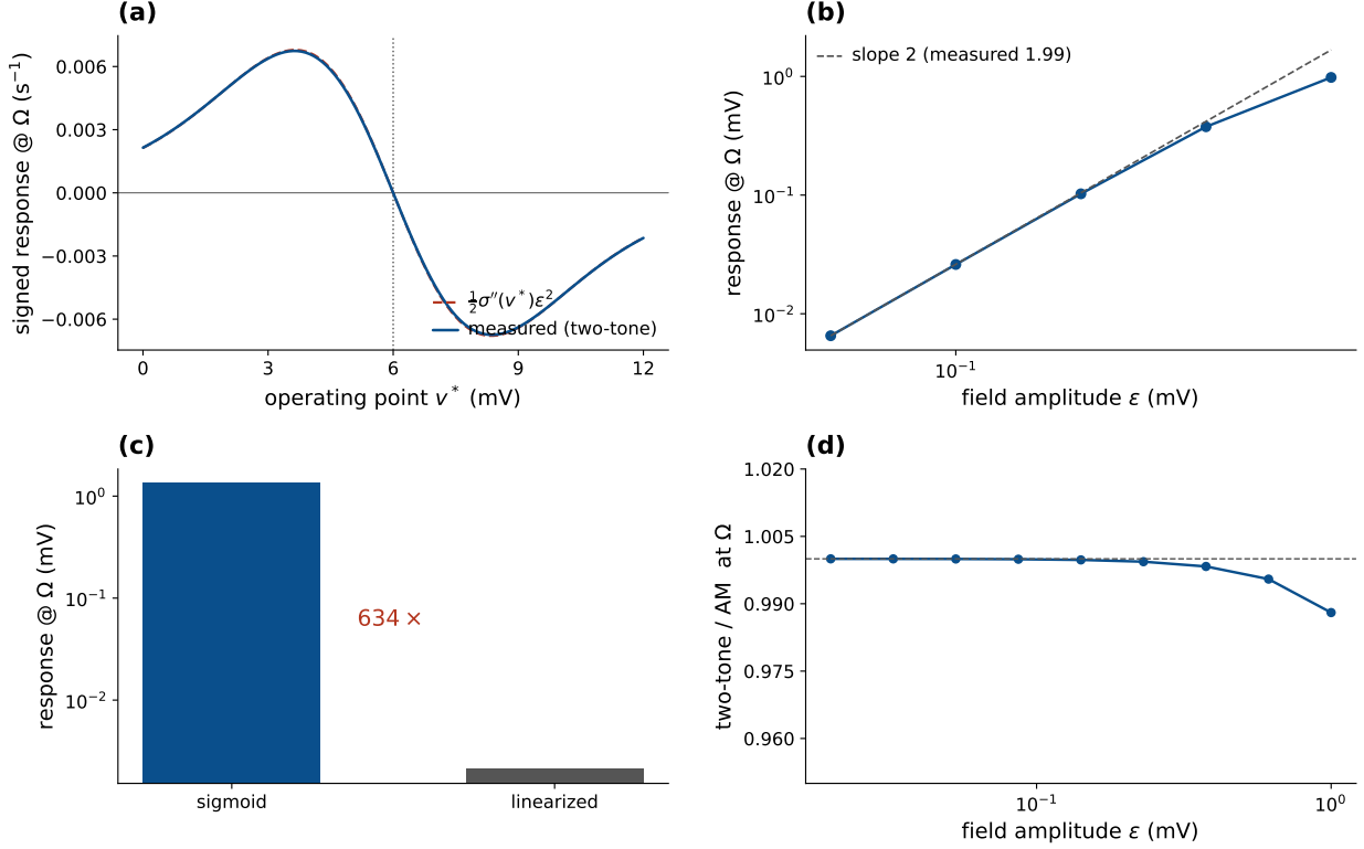
Figure 6: The curvature law, the square law, and the surrogate control (Jansen–Rit, genuine two tones). (a) The signed open-loop response tracks \frac{1}{2}\sigma''(v^*)\varepsilon^2 across the operating range (maximum deviation 0.9%), vanishing at the inflection v_0 and reversing sign across it. The mechanism is sign-agnostic: \sigma'' sets sign and phase while |\sigma''| sets gain, so the resonance picture is unchanged up to an overall sign in the \sigma'' > 0 lobe, which this sweep spans. The sign flip is itself a prediction (§4.10). (b) The closed-loop response scales as \varepsilon^2 , measured slope 1.99. (c) Replacing the field-receiving sigmoid by its tangent collapses the response 634 \times . (d) Surrogate control: the two-tone/AM ratio at \Omega approaches 1 as \varepsilon \rightarrow 0 (1.0000 at 0.02 mV, 0.988 at 1 mV), licensing the AM surrogate for the dense sweeps of Fig. 9, which read only that component, and for nothing else.
