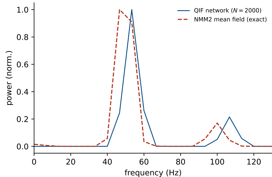
(a) QIF \rightarrow NMM2: matched gamma spectrum ( \langle r_E \rangle : 0.058 QIF vs 0.057 mean field)
