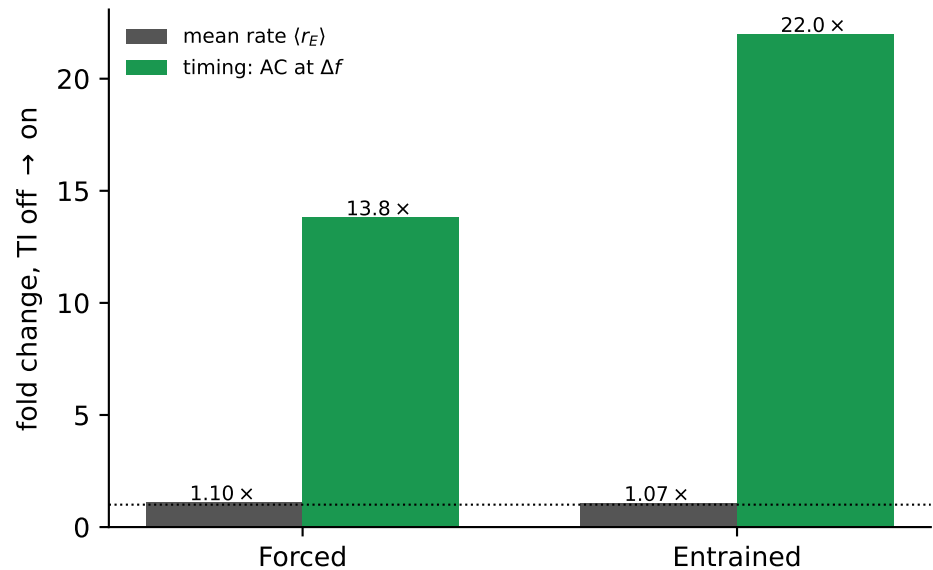
(b) TI multiplies envelope-locked timing, not the mean rate
