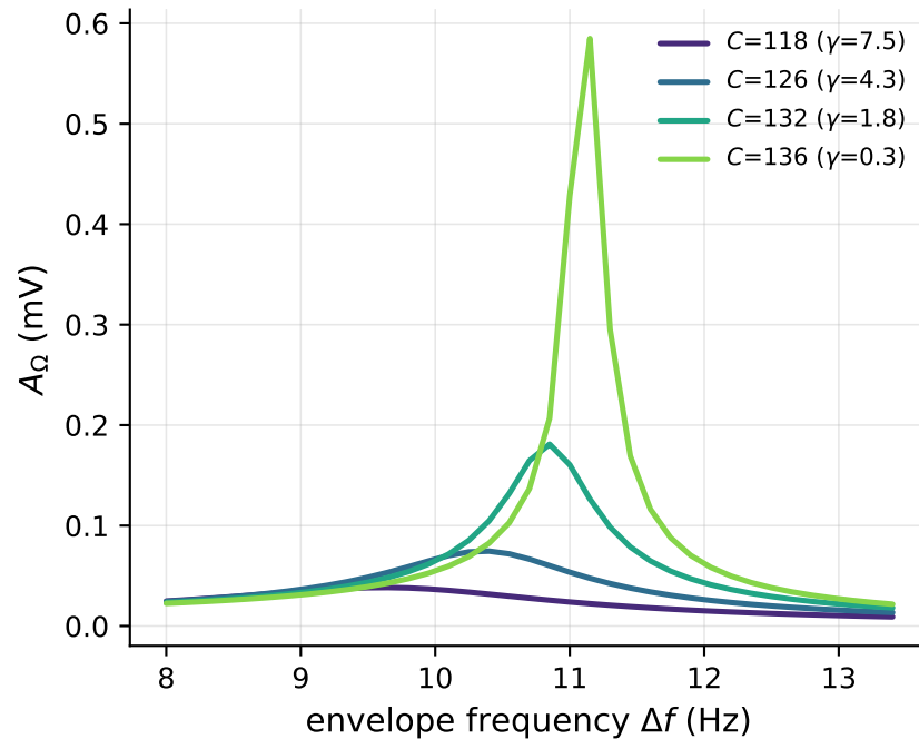
(b) resonance sharpens as C \rightarrow C^*
