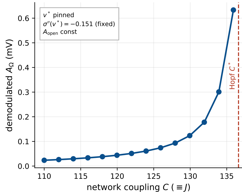
(a) the J curve
