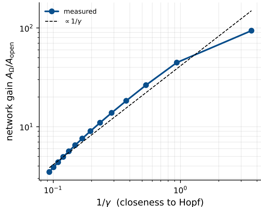
(c) gain \propto 1/\gamma , then saturates
