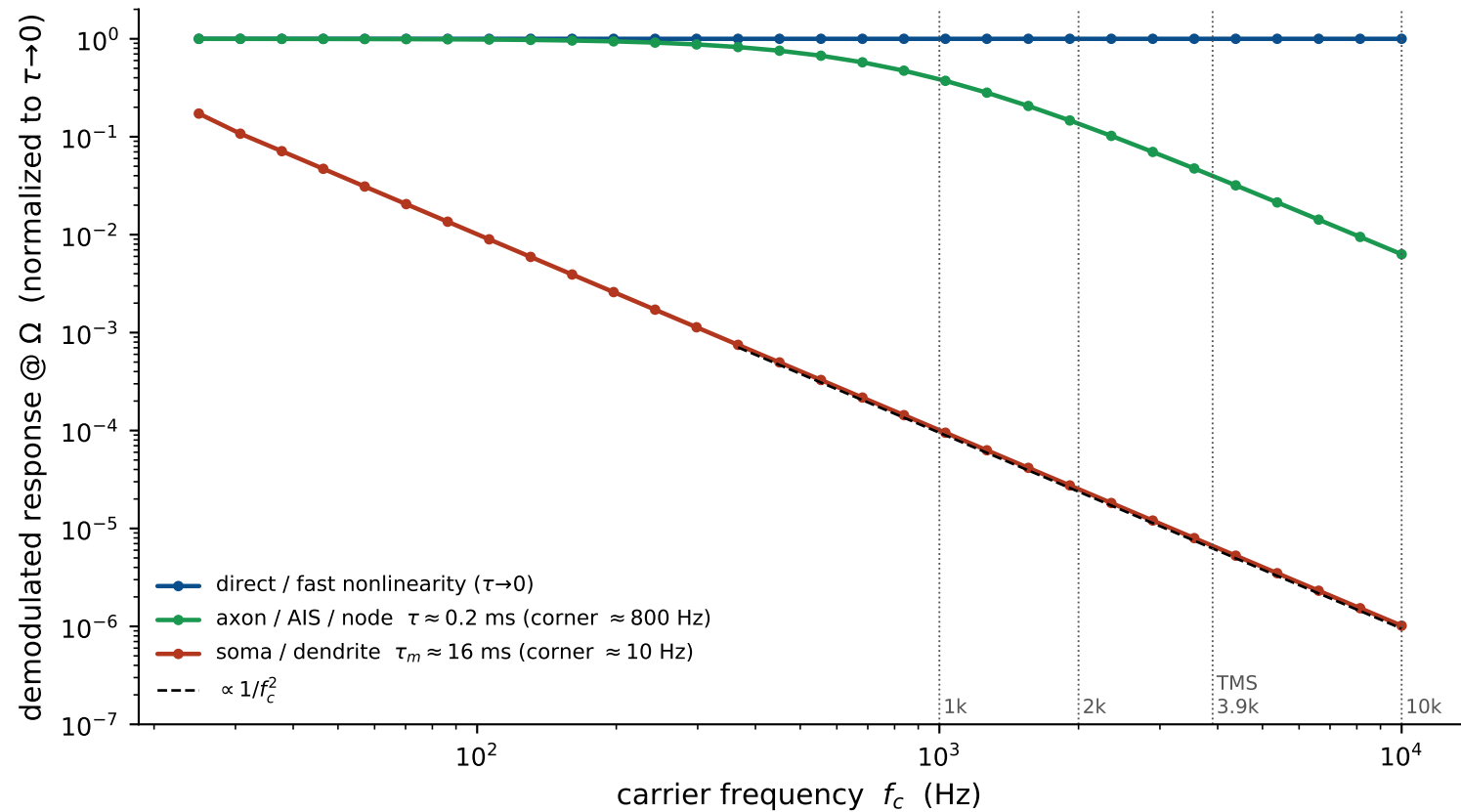
Where the nonlinearity sits decides kHz coupling (TI and TMS alike)
