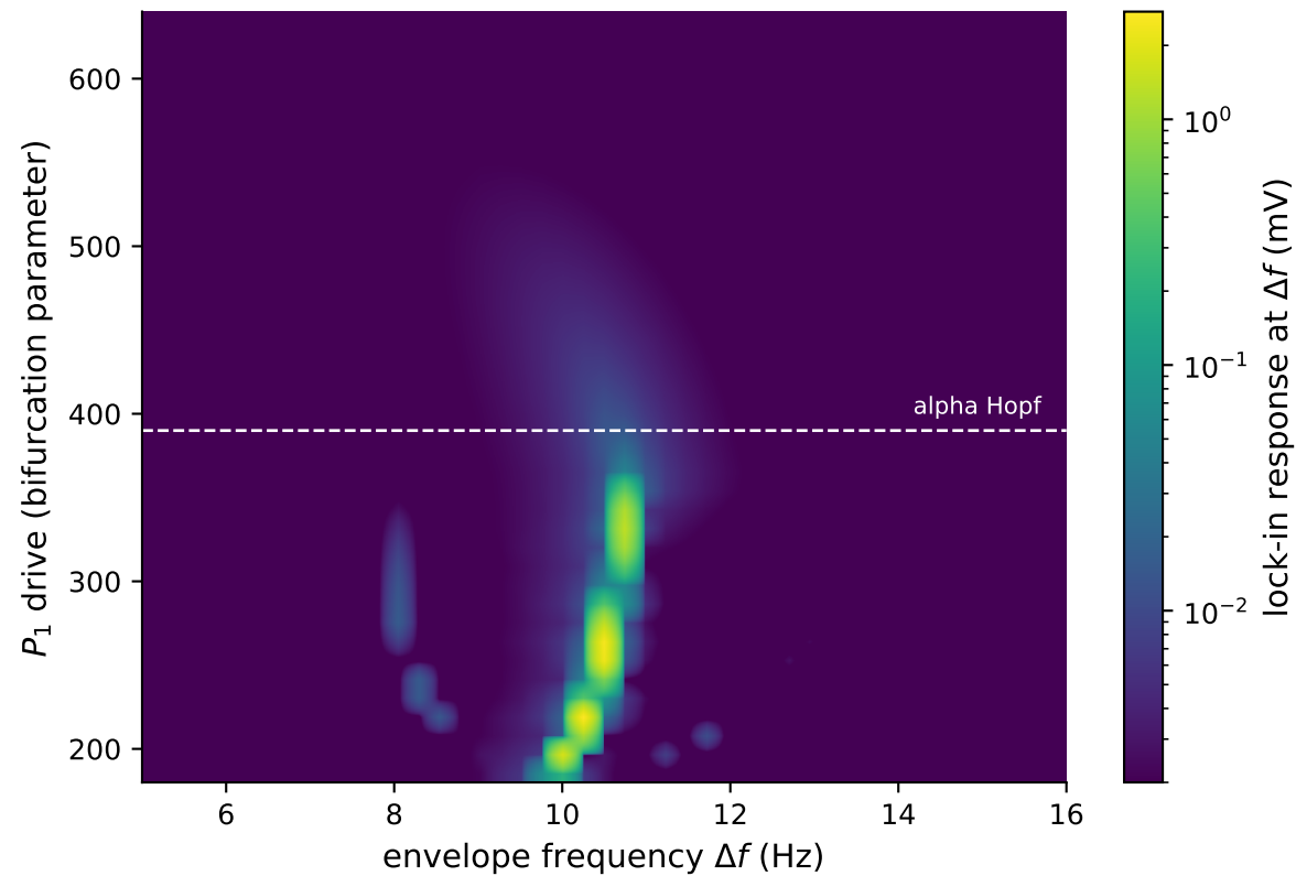
LaNMM: demodulated P_1 response over ( \Delta f , drive)
