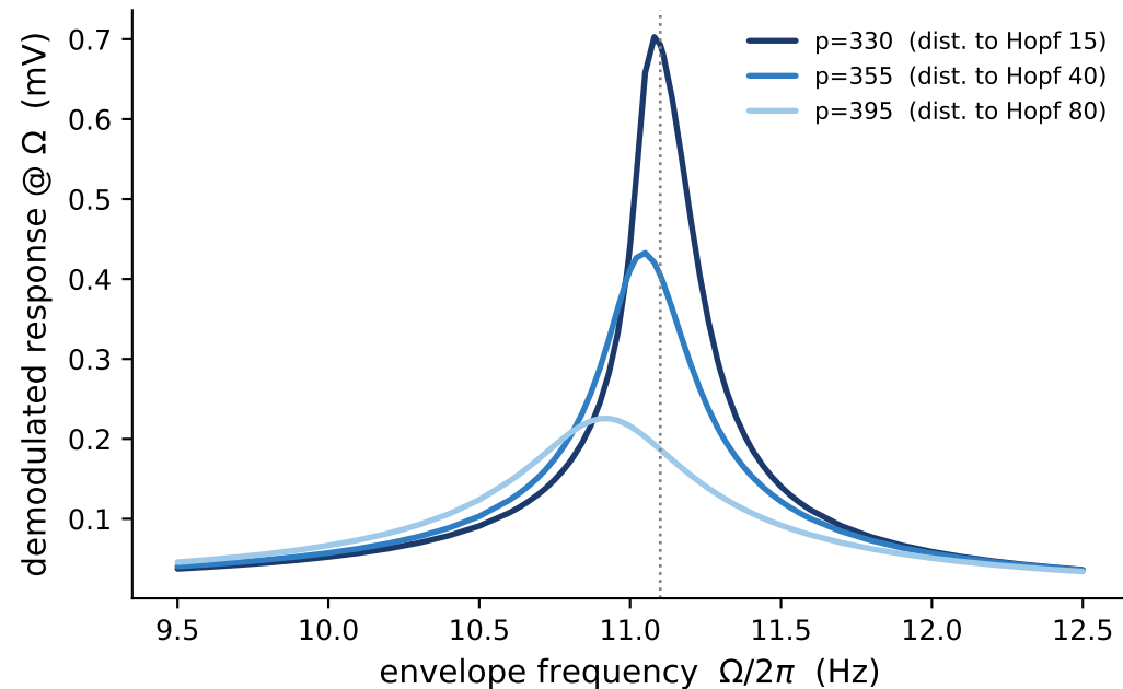
Stable focus (below Hopf): forced resonance
